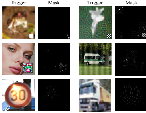
Figure 3: The poisoned images and the learned patches by DTINSPECTOR. The six examples correspond to six attacks, i.e., BADNET, TROJANN, CL, SIG, REFOOL, and FTROJAN, respectively.
