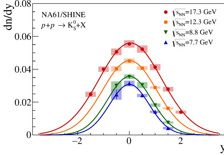
Figure 9: (Color online) Rapidity distribution dn/dy obtained by p_T -integration of data and extrapolation. Statistical uncertainties are shown by vertical bars (often smaller than the marker size), while shaded boxes indicate systematic uncertainties. The curves indicate the result of the Gaussian fit to the measured points. Points for p+p at \sqrt{s_{NN}} = 17.3 GeV are taken from [4].
