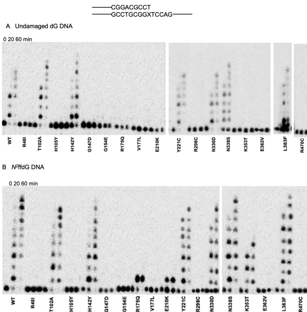
Figure 4. Primer extension in the presence of MatchT primer. DNA pol \kappa SNPs variants T102A, H142Y, Y221C, N330D, N338S, and L383F showed similar primer extension patterns in the presence of both undamaged (A) and minor groove damaged N^2 ffdG (B) DNA templates. Variants R175Q, E210K, and K353T showed primer extension only in the presence of damaged N^2 ffdG. Time points are 0, 20, and 60 min for each variant; quantitation is reported in Table S4, Figure S3.
