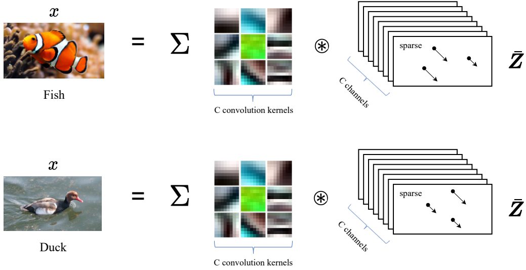
Figure 8: Each input signal x (an image here) can be represented as a superposition of sparse convolutions with multiple kernels d_c in a dictionary D .
