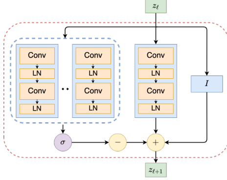
Figure 17: (Left) ReduNet-inspired architecture : Network architecture of convolutional ReduLayer, where each linear operator \mathbf{E}_\ell or \mathbf{C}_\ell^j is replaced by convolutions and layer normalization. (Right) Classification performance of ReduNet-inspired architecture on CIFAR10. ReLU indicates whether the (first layer of) the deep network architecture contains nonlinear ReLU activation or not.
