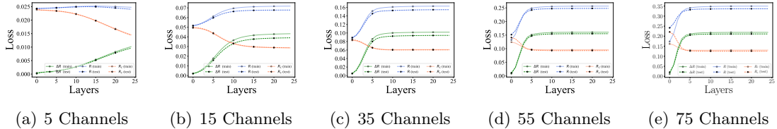
Figure 27: Training and test losses of translation invariant ReduNet for translation invariance on the MNIST dataset (TI-MNIST).
