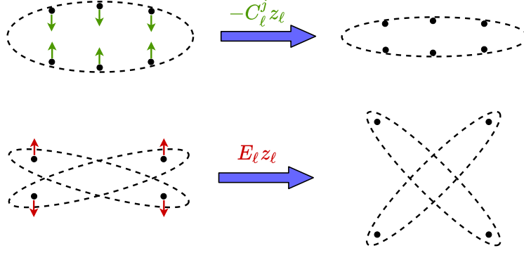
Figure 5: Interpretation of C_\ell^j and E_\ell : C_\ell^j compresses each class by contracting the features to a low-dimensional subspace; E_\ell expands all features by contrasting and repelling features across different classes.
