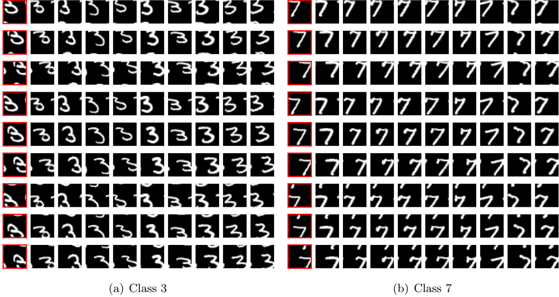
Figure 30: Verification of Equivariance in ReduNet. For each class of samples, and for all training samples (and their augmentations) \mathbf{z}^i and a test sample (and its augmentations) \hat{\mathbf{z}} , we compute their inner product |\langle \hat{\mathbf{z}}, \mathbf{z}^i \rangle| , \forall i . We select the top-9 largest inner products (sorted from left to right), and visualize their respective image. The test sample and its augmented version are highlighted in red.
