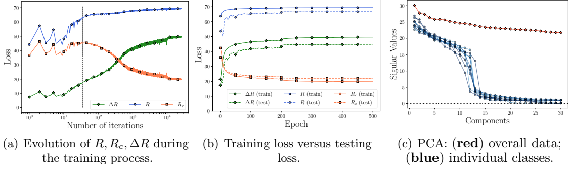
Figure 12: Evolution of the rates of \text{MCR}^2 in the training process and principal components of learned features.
