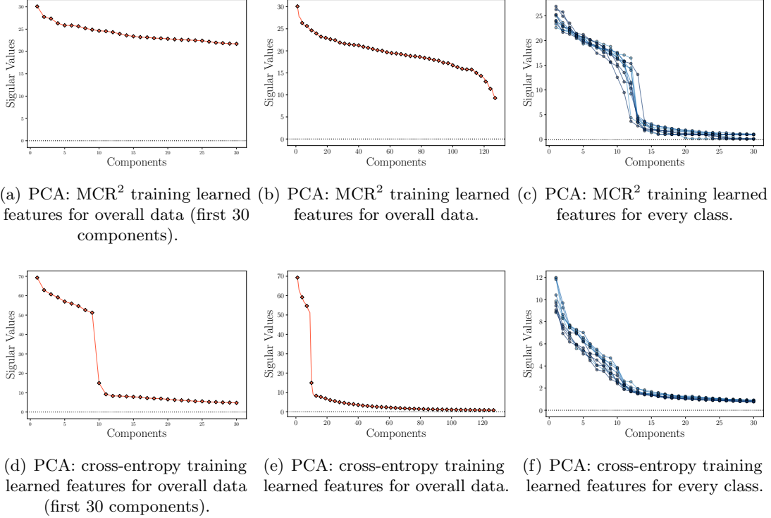
Figure 18: Principal component analysis (PCA) of learned representations for the \text{MCR}^2 trained model ( first row ) and the cross-entropy trained model ( second row ).
