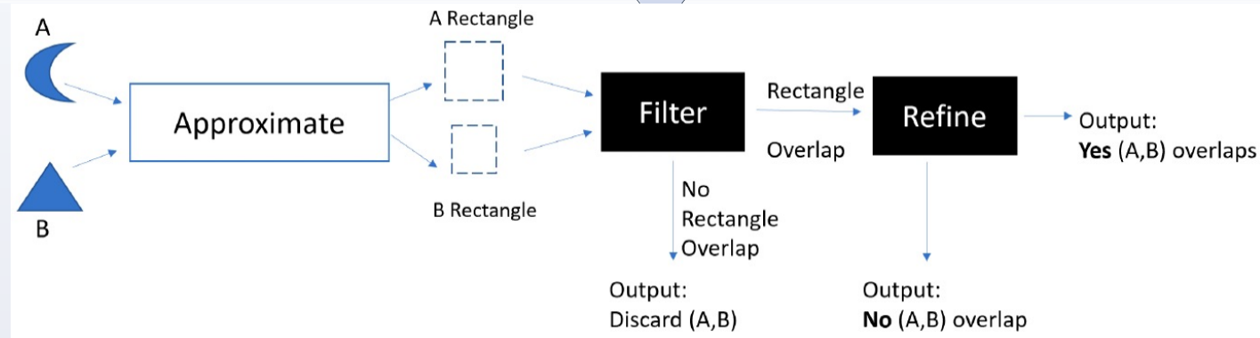
Fig. 2 Filter and refine for two input polygons using their rectangles. Only those pairs (A,B) will pass the filter if their rectangle approximations overlap. Spatial join processes millions of such pairs.
