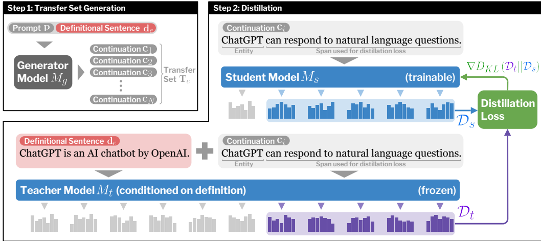
Figure 1: Overview of our distillation approach. Our goal is to inject the entity definition ( d_e ) into the student model ( M_s ) and propagate it to make inferences based on the injected knowledge. This example uses ChatGPT as a new entity. We first generate a set of continuations of the entity’s definition using a generator model (Step 1), then use these to distill the information from definition into the student model via a KL loss between the conditioned and unconditioned models (Step 2); see Section 3 for formulation.
