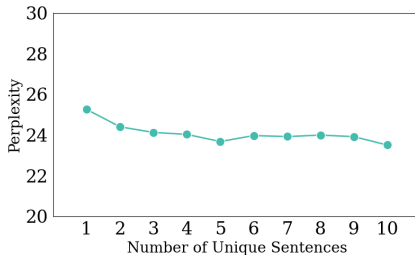
Figure 5: Perplexity for using n distinct transfer sentences during distillation, with number of updates standardized to 10. We see the benefit of having a diverse transfer set compared to repeating the same transfer sentence 10 times.
