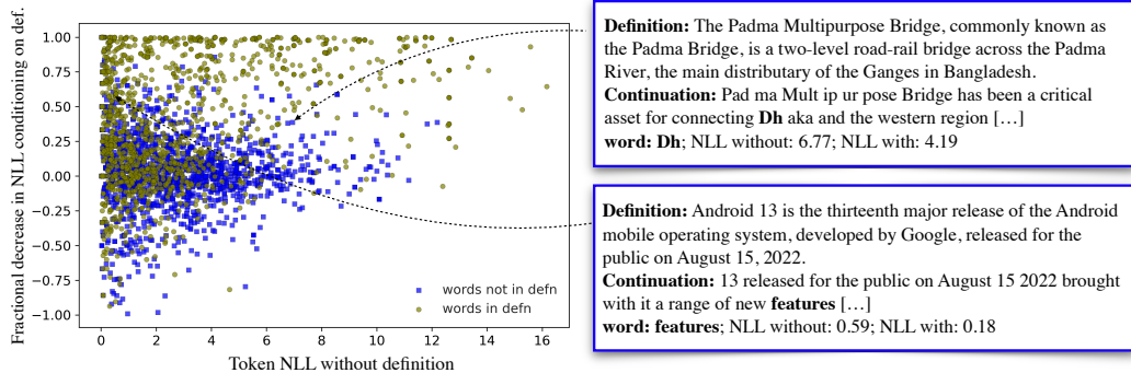
Figure 3: Per-token NLL of tokens in continuations before conditioning on definitions and after (fractional reduction). Tokens not in the definition (blue dots) are changed less but do see lower NLL when they are inferable from the definition (examples).
