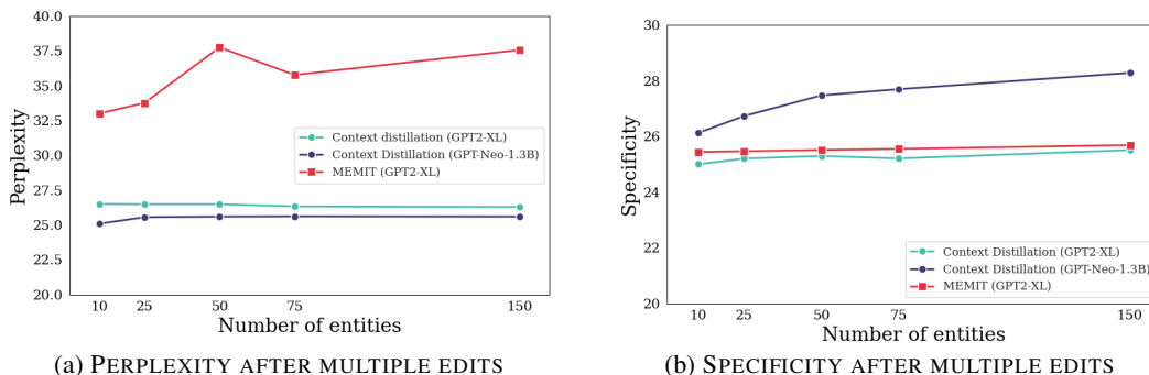
Figure 4: Editing for multiple entities at once. We report the average from three runs with different random seeds for shuffling training data.
