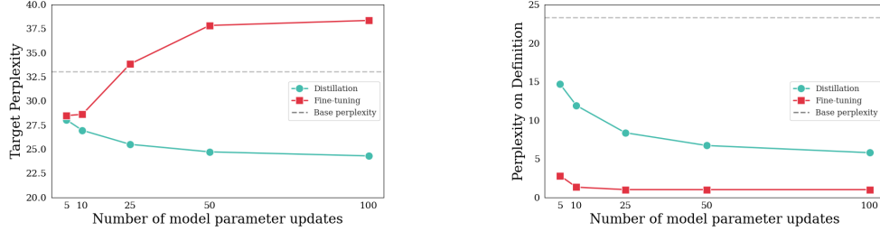
Figure 2: Results on GPT-Neo with varying numbers of model updates for fine-tuning and distillation approach. Left: target perplexity; right: perplexity on the definition sentence. Only distillation continues to improve in both target and definition perplexity as the number of updates increase.
