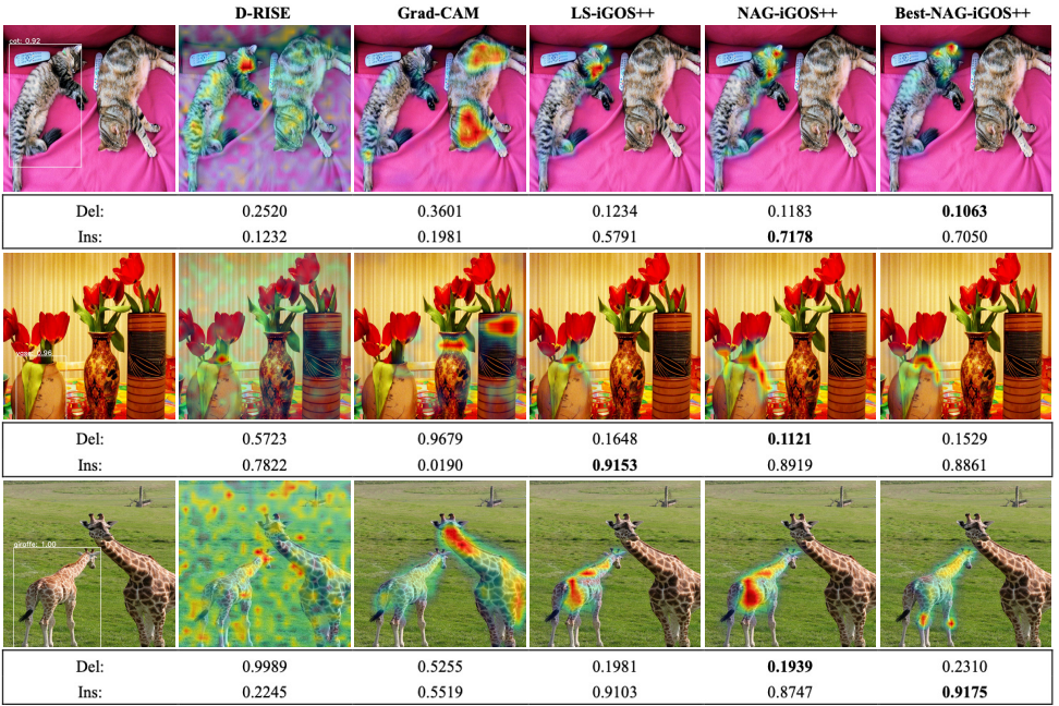
Figure 3: Visualization of the heatmap generated from different methods at the 25x25 resolution on Mask R-CNN detections
