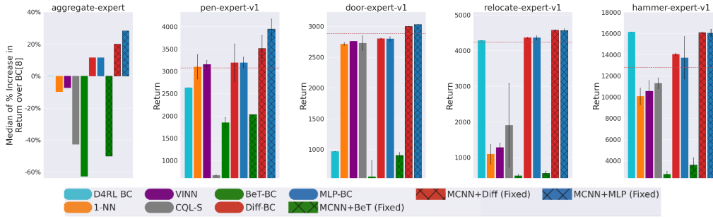
Figure 5: Adroit expert tasks [5000 demos] : Comparison of returns (across 20 evaluation trajectories and 3 random seeds) between baselines and our methods (MCNN+BeT, MCNN+Diff, and MCNN+MLP). Our MCNN methods use the same fixed set of hyperparameters across all tasks.
