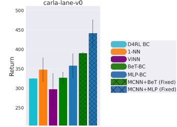
Figure 8: CARLA [400 demos] : Comparison of return (across 20 evaluation trajectories and 3 random seeds) between baselines and our methods (MCNN+BeT and MCNN+MLP). For the results shown here, our MCNN methods use the same fixed set of hyperparameters across all tasks.
