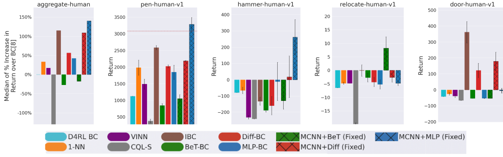
Figure 4: Adroit human tasks [25 demos] : Comparison of returns (across 20 evaluation trajectories and 3 random seeds) between baselines and our methods (MCNN+BeT, MCNN+Diff, and MCNN+MLP). Our MCNN methods use the same fixed set of hyperparameters across all tasks.
