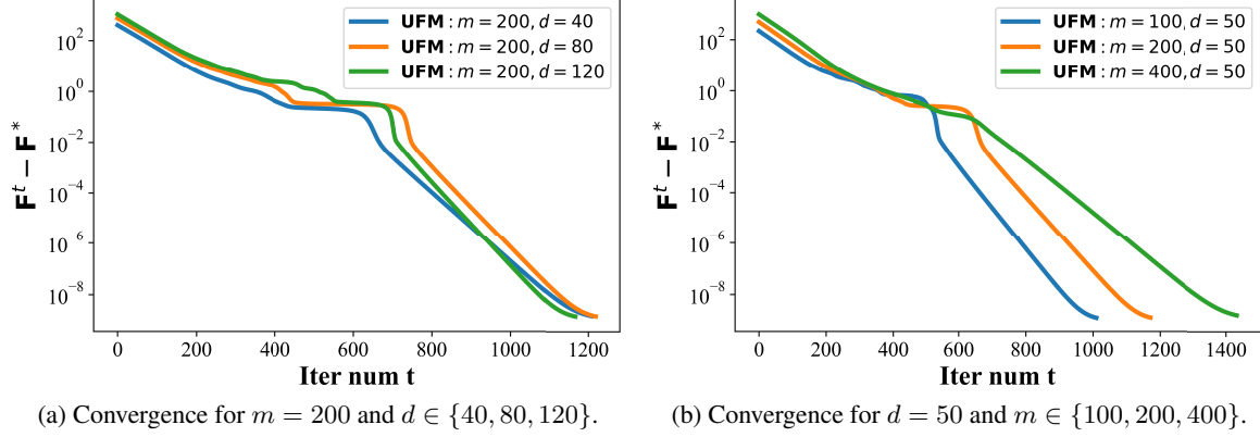
Figure 3. Convergence performance of GD for solving the regularized MCR 2 problem. The x -axis is number of iterations (also denoted by t ), and the y -axis is the function value gap F^t - F^* , where F^t = F(\mathbf{Z}^t) denotes the function value at the t -th iterate \mathbf{Z}^t generated by GD, and F^* is the optimal value of Problem (5) computed according to (7) in Theorem 3.1.
