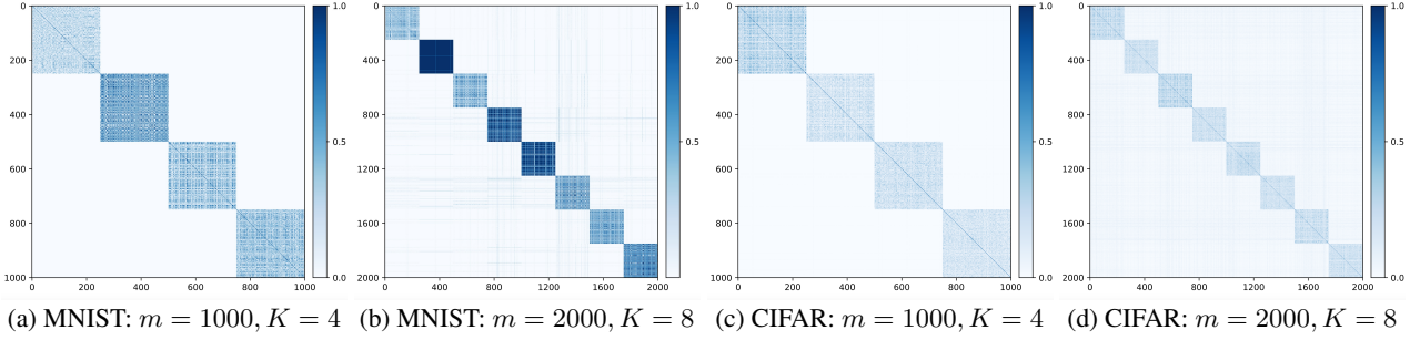
Figure 9. Heatmap of cosine similarity among learned features by training deep networks on MNIST and CIFAR-10. We train network parameters by optimizing the regularized MCR 2 objective (5) on m samples split equally among K classes of MNIST and CIFAR-10. In the figure, the darker pixels represent higher cosine similarity between features. In particular, when the (i, j) -th pixel is close to 0 (very light blue), the features i and j are approximately orthogonal.
