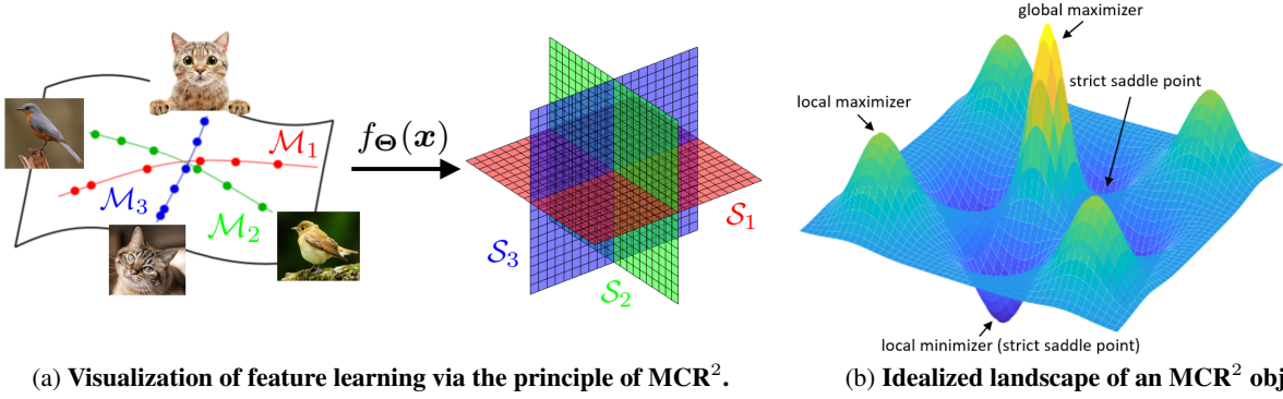
Figure 1. An illustration of the properties of \text{MCR}^2 . (a) The high-dimensional data \{x_i\} \subseteq \mathbb{R}^n lies on a union of low-dimensional submanifolds. The objective of \text{MCR}^2 is to learn a feature mapping f_\Theta(\cdot) : \mathbb{R}^n \rightarrow \mathbb{R}^d such that z_i = f_\Theta(x_i) for all i are low-dimensional, discriminative, and diverse. (b) According to Theorems 3.1 and 3.3, the regularized \text{MCR}^2 problem has a benign optimization landscape: each critical point is either a local maximizer or a strict saddle point. Furthermore, each local maximizer, just like the global maximizer, corresponds to a feature representation that consists of a family of orthogonal subspaces, as illustrated in the middle.
