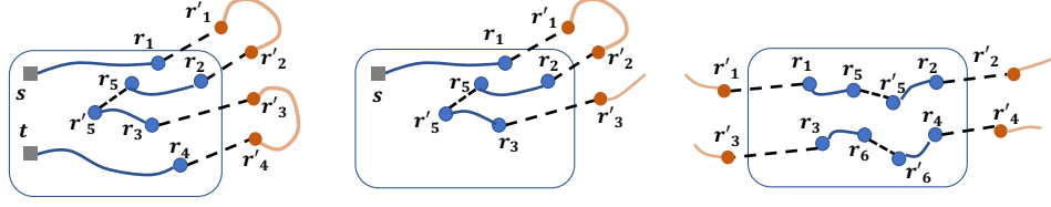
Figure 2: Examples of compact subgraphs and anchor edges in the algorithm for computing higher-order sensitivity of paths: (Left) D = \{r_1, r_2, r_3, r_4\} , edges (r_1, r'_1) , (r_2, r'_2) , (r_3, r'_3) and (r_4, r'_4) are external anchor edges, while (r_5, r'_5) is an internal anchor edge. Nodes s and t are the starting and ending nodes of the path; (Middle) D = \{r_1, r_2, r_3\} , and (r_1, r'_1) , (r_2, r'_2) , (r_3, r'_3) are external anchor edges, while (r_5, r'_5) is an internal anchor edge. Node s is the starting node of the path, and the path ends at some other node, not in this compact subgraph; (Right) D = \{r_1, r_2, r_3, r_4\} , edges (r_1, r'_1) , (r_2, r'_2) , (r_3, r'_3) and (r_4, r'_4) are external anchor edges, while (r_5, r'_5) and (r_6, r'_6) are internal anchor edges. Paths pass through this compact subgraph, without starting or ending in it.
