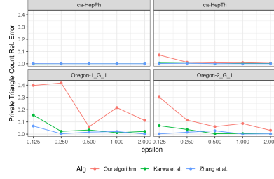
Figure 3: Triangle Count Relative Error, showing the accuracy of the private triangle count with noise calibrated by (1) our approximate smooth sensitivity (Algorithm 2), (2) the exact smooth sensitivity (Karwa et al.), and (3) the ladder function (Zhang et al.)
