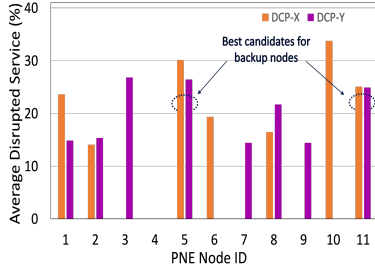
Fig. 3: Impact of PNE-node failure.
