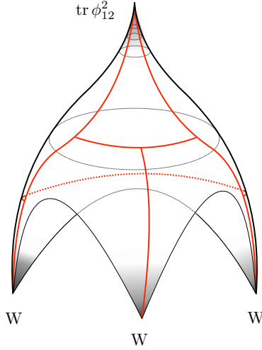
Figure 3. World-sheet perspective of the three-leg form factor and the non-planar graph from Fig. 2 (d) overlayed on it: it demonstrates why it produces contribution of leading order in color.
