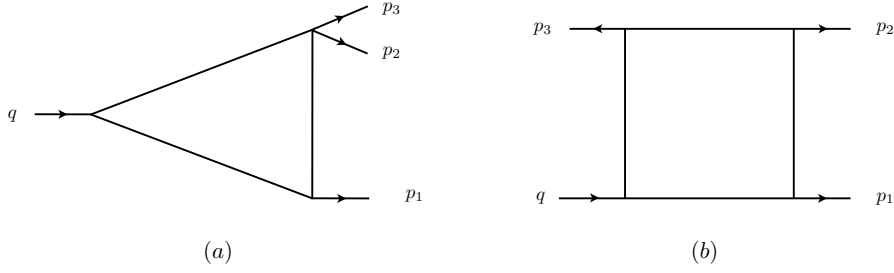
Figure 1. Graphs contributing to the one-loop form factor F_3^{(1)} .
