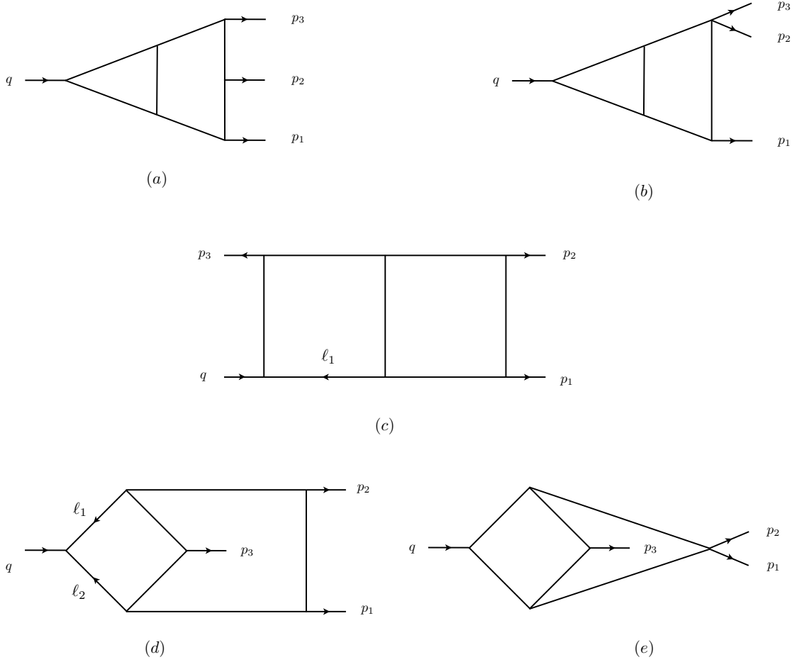
Figure 2. Graphs contributing to the two-loop form factor F_3^{(2)} . The integrands, built from product of propagators read off from these diagrams, are accompanied by numerators according to Eqs. (4.1)–(4.5).
