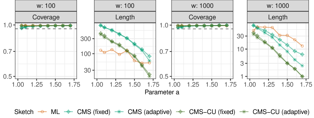
Figure A22: Performance of 95% confidence intervals based on different data sketches, either with width w = 100 or w = 1000 . The results are shown as a function of the tail parameter of the Zipf distribution from which the data are sampled. The conformity scores are evaluated separately within L = 5 frequency bins, seeking frequency-range conditional coverage (10). Other details are as in Figure A21.
