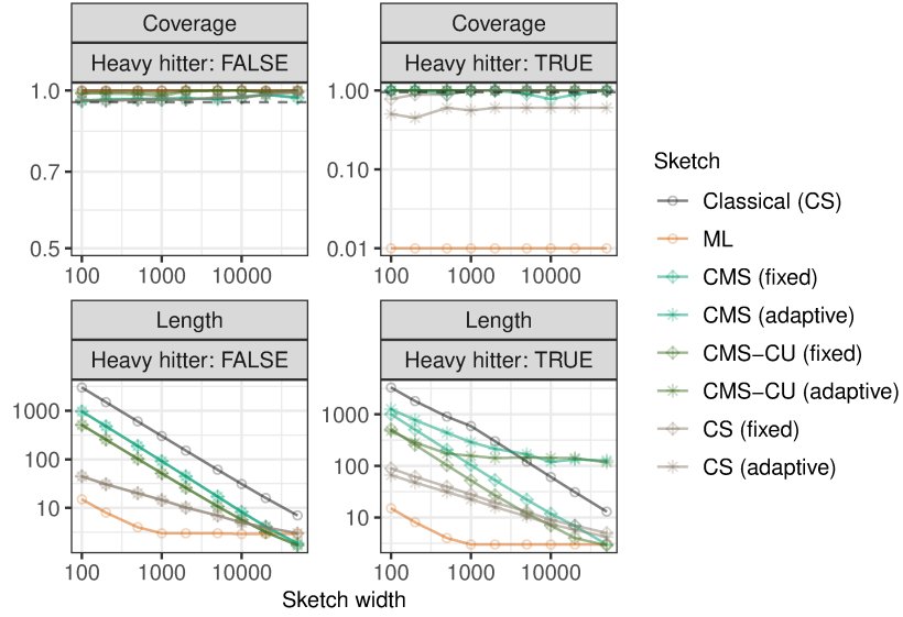
Figure A28: Performance of 95% confidence intervals for random queries, based on synthetic data with heavy hitters. The coverage and average width of the conformal confidence intervals is reported separately for heavy hitters and all other objects. Other details are as in Figure A27. These results show that the CS sketch applied in combination with our method leads to the most informative confidence intervals—it achieves shorter width while ensuring valid coverage conditional on whether the queried object is a heavy hitter. Note that the true conditional coverage obtained with ML sketch for heavy hitter queries is zero, even though a truncated value of 0.01 is shown on the logarithmic scale for convenience.
