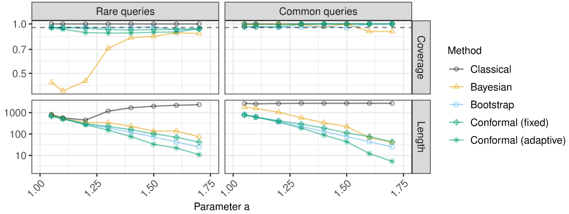
Figure A11: Performance of confidence intervals stratified by the true query frequency. Left: frequency below median; right: above median. Here, the conformal confidence intervals are constructed using Algorithm 2, which seeks marginal coverage (2), instead of Algorithm 3, which seeks frequency-range conditional coverage (10). Other details are as in Figure 3.
