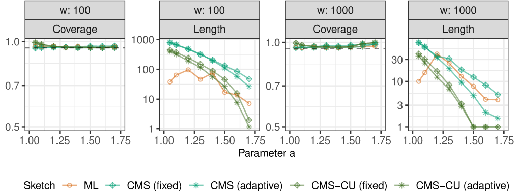
Figure A21: Performance of 95% confidence intervals based on different data sketches, either with width w = 100 or w = 1000 . The results are shown as a function of the tail parameter of the Zipf distribution from which the data are sampled. Other details are as in Figure 7.
