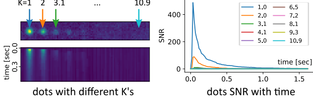
Figure 4. Laser dot projection times. (Left) A thermal image showing the relative intensity of laser dots projected at different durations T^{\text{smp}}/K , where K is the number of points per frame. Below is a plot of a single row over time (vertically). (Right) Dot SNR over time for various K .
