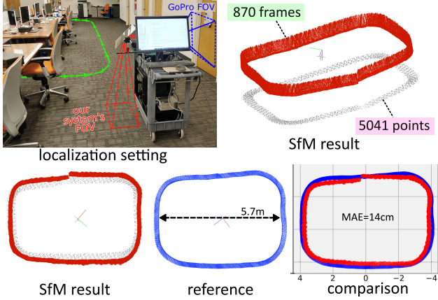
Figure 9. Indoor localization. We loop around office desks while pointing the system towards the floor. Our method yields accurate tracks and loop closure, with no shared feature points between the first and last frames. The blue reference camera poses stem from a COLMAP reconstruction using frames from a GoPro camera affixed to the cart’s outer end, pointed at the office.
