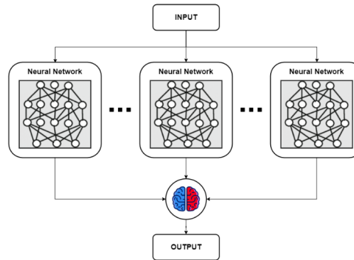
Figure 9: Diagram of the flow of an ensemble neural network. Each individual network receives the same input but produces their own output which is later combined for a final prediction.
