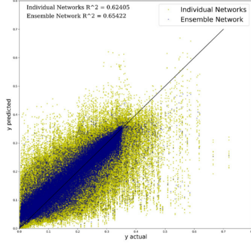
Figure 18: Scatter plot error visualization comparison of individual network predictions and the averaged ensemble neural network's final prediction with associated R^2 and mean squared error values.
