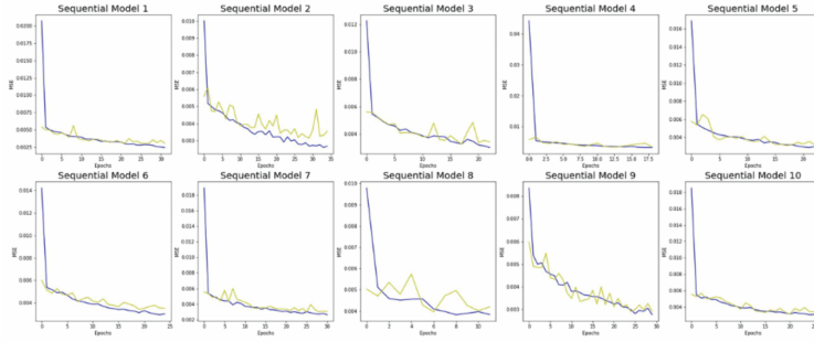
Figure 10: Mean squared error of training (blue) and testing (yellow) data of ensemble. Visual representation of how each individual network is being trained differently.
