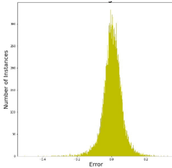
Figure 12: Histogram distance error visualization for single neural network predictions with overall mean squared error value.
