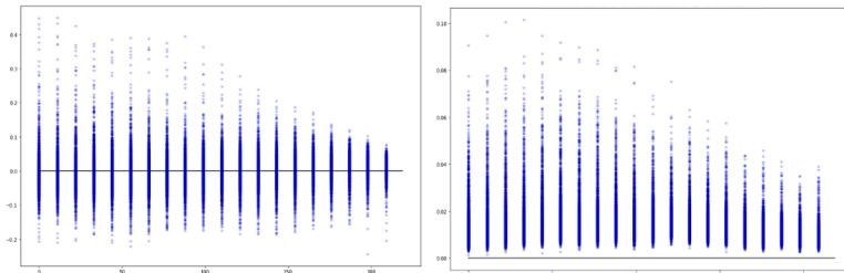
Figure 20: Comparison of point-wise error in each of the 20 points in each 2,000 predictions (left) to the point wise standard deviation of the 20 points in each 2,000 predictions (right) in the ensemble network.
