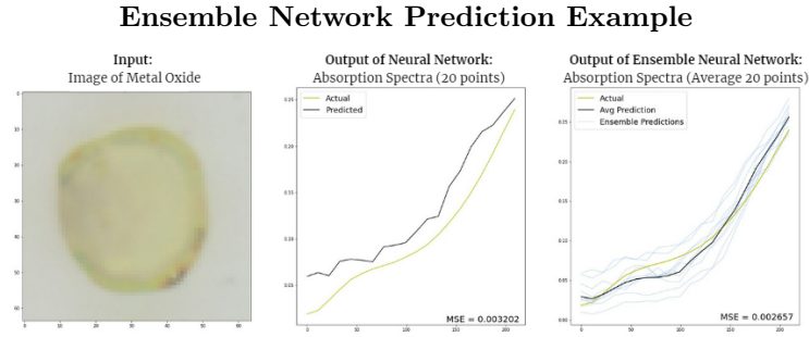
Figure 14: Comparison of 10 individual network predictions, the averaged ensemble prediction, and ground truth spectra for a singular spectra image.
