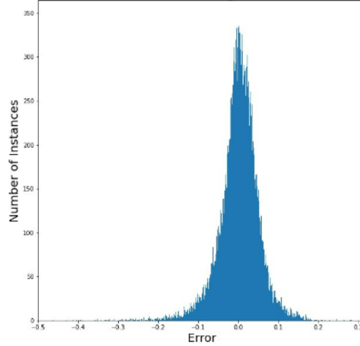
Figure 15: Histogram distance error visualization for an ensemble neural network predictions.
