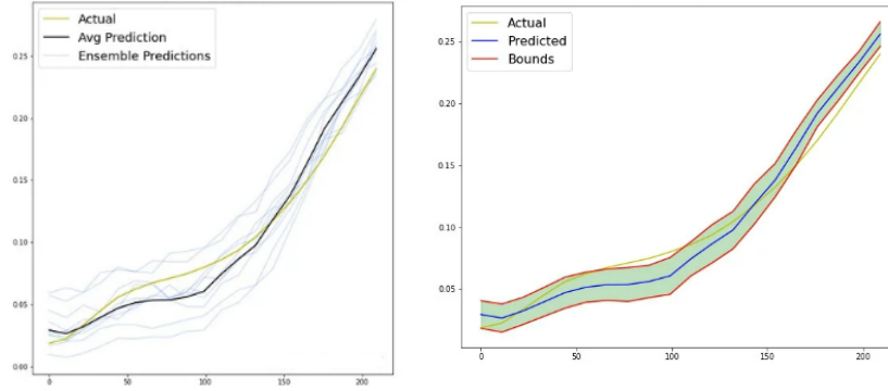
Figure 19: Comparison of individual network predictions (left) with changing area of a confidence interval (right).
