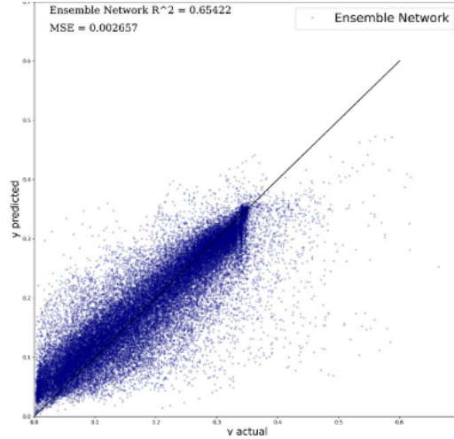
Figure 16: Scatter plot error visualization for an ensemble neural network predictions with R^2 value.
