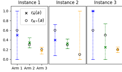
Figure 2: Representative draws of \mathcal{D}^{\text{off}} in our three Bernoulli MAB case studies, with parameters in Table 1. The dashed lines display the rectangular version space \mathcal{M}_{\delta'}(\mathcal{D}^{\text{off}}) with \delta' = 0.05 .
