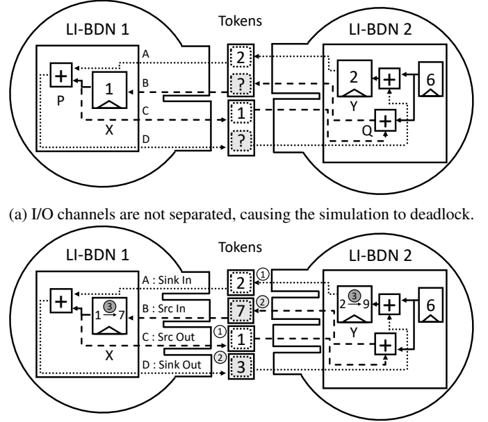
(a) I/O channels are not separated, causing the simulation to deadlock. (b) I/O channels are separated, enabling the simulation to make forward progress even though the partition boundary contains combinational logic.
