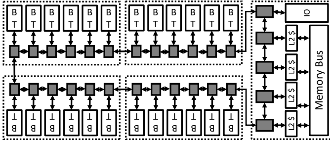
Fig. 6: 24 core SoC partition. We partition an SoC containing 24 BOOM tiles (BT) onto 5 FPGAs by utilizing the NoC-partition-mode . The entire simulation runs at 0.58 MHz.
