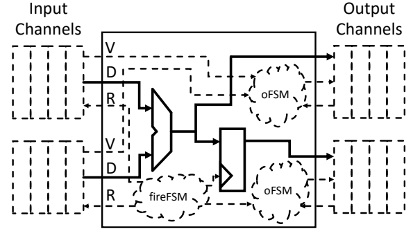
Fig. 1: LI-BDN. The solid lines indicate the original circuit while the dotted lines are extra circuitry added to generate the LI-BDN.
