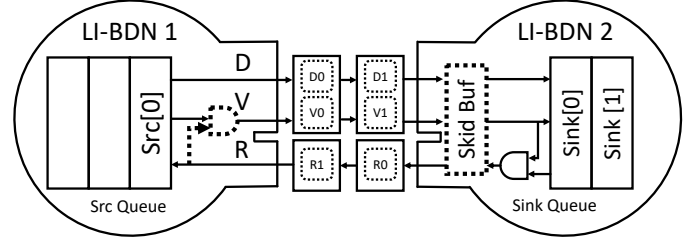
(c) Modifying the target boundary to preserve backpressure on a ready-valid interface.
