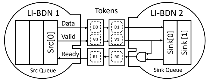
(a) Fast-mode without module boundary modifications.
