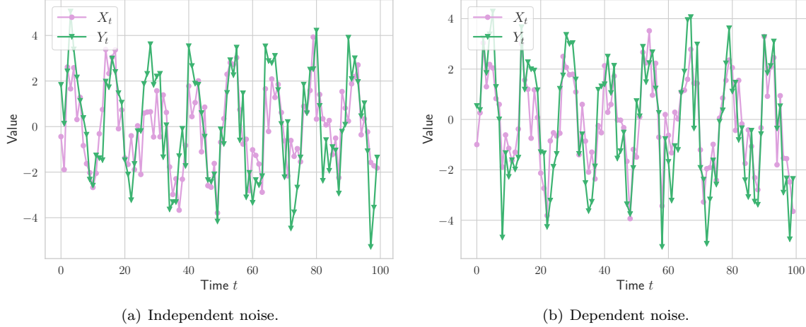
Figure 10: Sample of independent (subplot (a)) and dependent ( \rho = 0.5 , subplot(b)) data according to 3. The purpose of visualizing raw data is to demonstrate that dependence is hard to detect visually, and dependence refers to more than temporal correlation which may be present due to cyclical trends.
