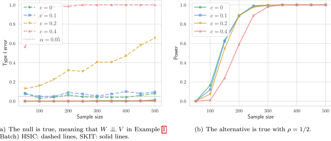
Figure 2: Under distribution drift (3), SKIT controls type I error under H_0 and has high power under H_1 . Batch HSIC fails to control type I error under H_0 (hence we do not plot its power).
