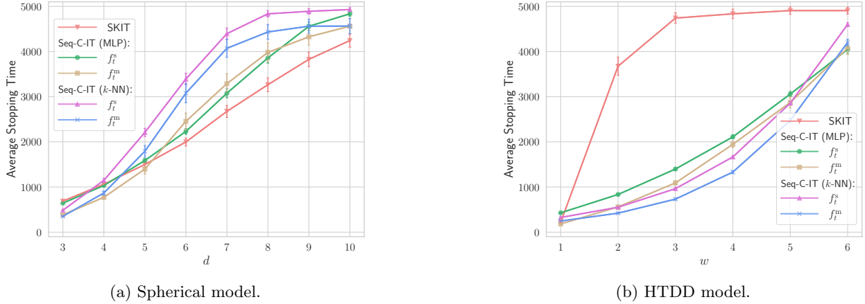
Figure 7: Stopping times of ITs on synthetic data from Section 3. Subplot (a) shows that SKIT is only marginally better than Seq-C-IT (MLP) due to slightly better sample efficiency under the spherical model (no localized dependence). Under the structured HTDD model, SKIT is inferior to Seq-C-ITs.
