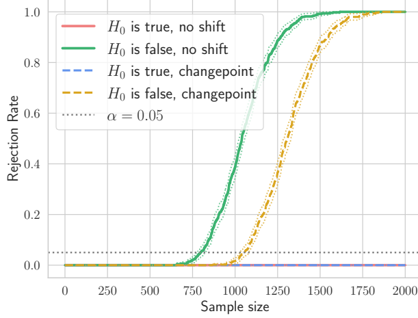
Figure 6: Average rejection rates for four settings: solid lines correspond to the standard i.i.d. setting and dashed lines correspond to the settings that involve distribution shift. Despite there being a shift in distribution, our test that utilizes logistic regression learned via online gradient descent controls the type-1 error under a more general 2ST null hypothesis and has power under the alternative. Results are aggregated over 500 random sequences from the corresponding distributions.
