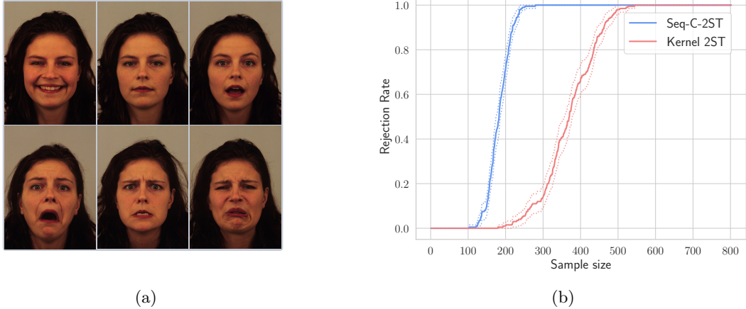
Figure 3: (a) Examples of instances from P (top row) and Q (bottom row) for KDEF dataset. (b) Rejection rates for our test (Seq-C-2ST) and the sequential kernelized 2ST. While both tests achieve perfect power with enough data, our test is superior to the kernelized approach, requiring fewer observations to do so. The results are averaged over 200 random orderings of the data.
