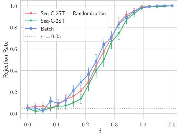
Figure 9: Comparison between the batch and sequential 2STs on Gaussian data when the sample size is set beforehand to 1500. First, invoking randomization improves the power of our sequential test across all settings. Second, batch 2ST has only slightly higher power across many settings. Note that the power of Seq-C-2ST can be easily improved after collecting a bit more data, yet this is not allowed for the batch test.
