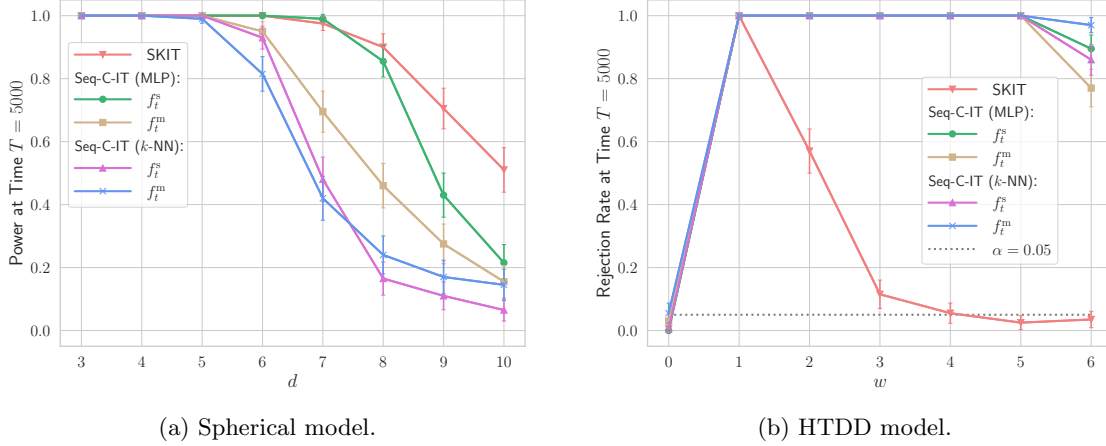
Figure 2: Power of different sequential independence tests on synthetic data from Section 3. Under the spherical model (no localized dependence), SKIT is better than Seq-C-ITs. Under the (structured) HTDD model, SKIT is inferior to sequential predictive independence tests.
