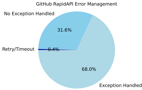
Fig. 10: Error Handling Code Patterns
