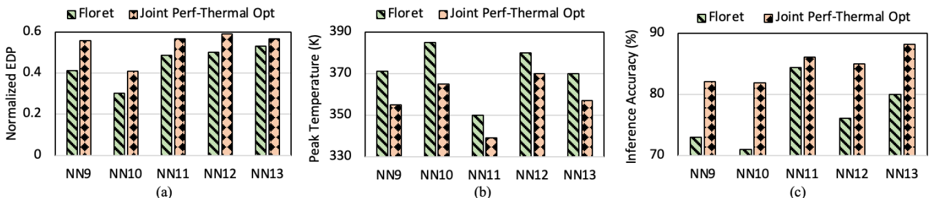
Fig. 6: (a) EDP comparison; (b) Peak temperature comparison; (c) Impact on DNN inference accuracy due to thermal noise on 100 PE NoC-enabled 3D system. Authorized licensed use limited to: Washington State University. Downloaded on July 08, 2024 at 16:53:02 UTC from IEEE Xplore. Restrictions apply.
