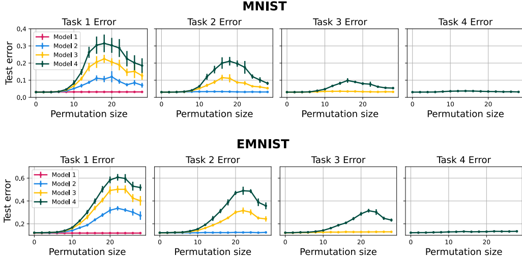
Figure 6: Results of the permutation experiment for varying levels of permutation size. The architecture is a 2-layer MLP of width 400. Model 1 corresponds to the net that is trained on task 1, Model 2 corresponds to the net that is trained on task 1 then task 2, and so on. Plotted curves have been averaged over 10 runs and error bars denote standard deviation of test error over the runs.
