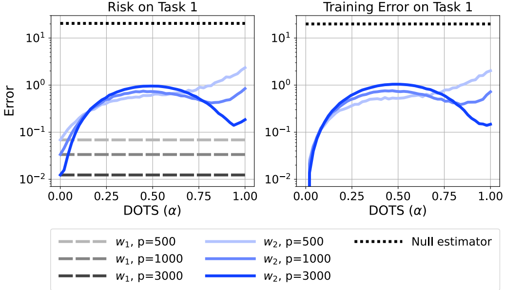
Figure 4: Results of the numerical simulation. Risk and training error on task 1 are plotted as a function of \alpha for various levels of p . The solid (blue) curves denote performance on task 1 of an estimator that is trained on task 1 and then on task 2. The dashed dark lines denote performance on task 1 of an estimator trained on task 1 only. The dotted black line denotes the performance of the null estimator. Training error curves for w_1 are omitted as these values are 0 for p > d .
