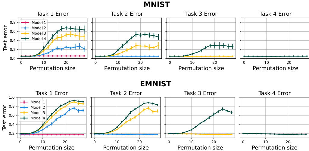
Figure 7: Replication of the experiment in Figure 6 using less overparameterized 2-layer MLP models (width 20 for MNIST and width 40 for EMNIST).
