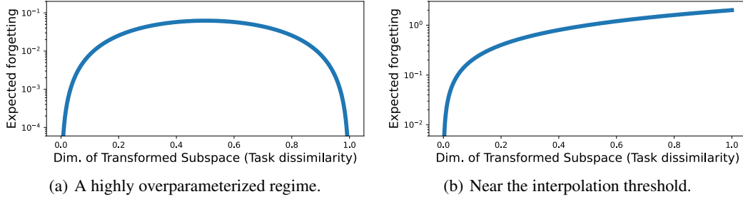
Figure 1: Informal illustration of our theoretical result. Formal details are shared in Section 2
