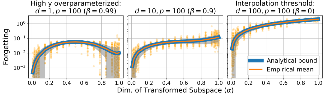
Figure 2: Empirically illustrating the worst-case forgetting under different overparameterization levels. Points indicate the forgetting under 1000 sampled random transformations applied on a (single) random data matrix \mathbf{X} . Their mean is shown in the thin orange line, with the standard deviation represented by a gray band. The thick blue line depicts the analytical expression of Theorem 3. Here, we restrict the nonzero singular values of \mathbf{X} to be identical, saturating the inequality in Eq. (4). Indeed, the analytical bound matches the empirical mean, thus exemplifying the tightness of our analysis. For completeness, in Appendix C.3 we repeat this experiment with p = 10 and p = 1000 .
