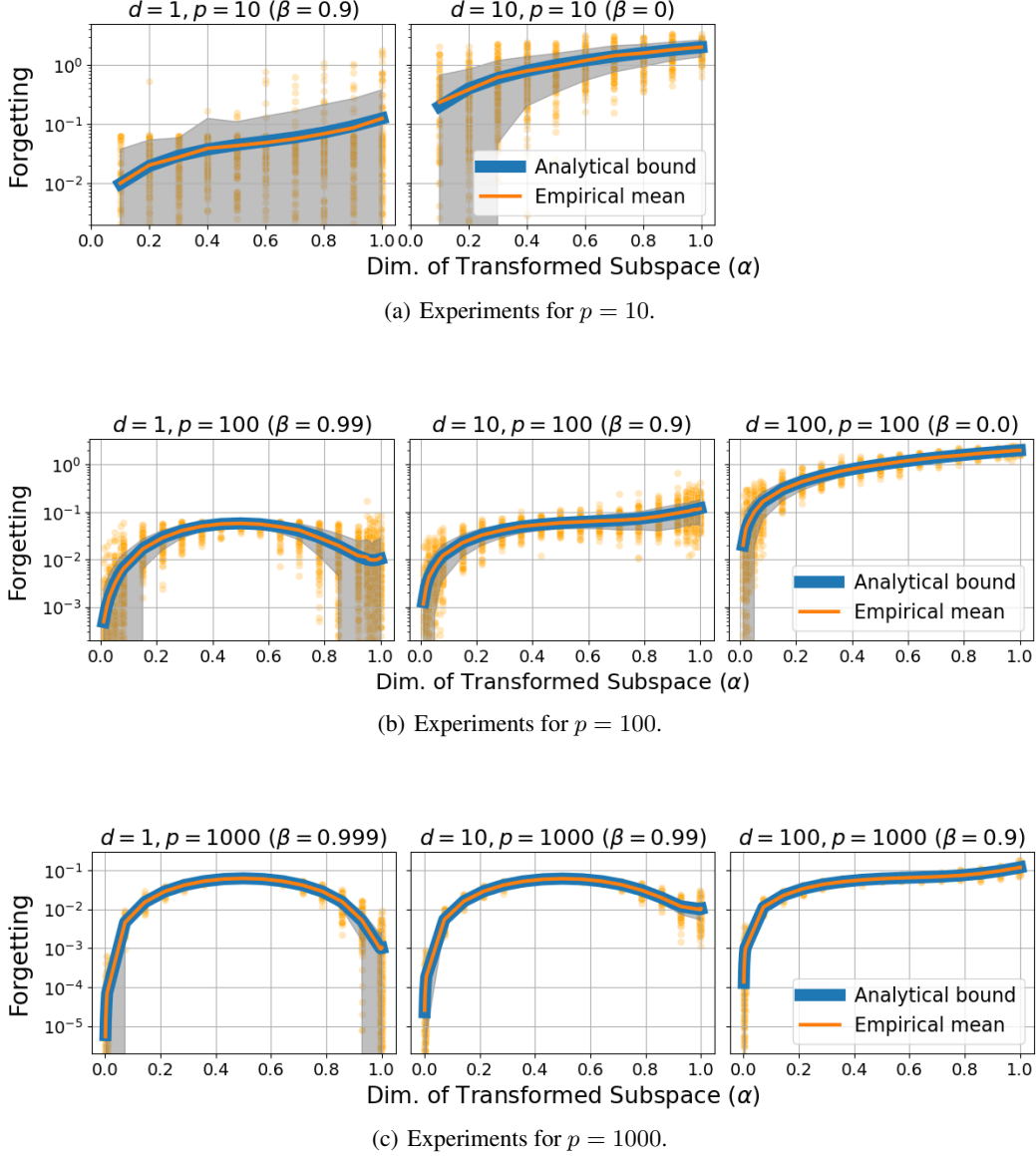
Figure 9: Empirically illustrating the worst-case forgetting under different overparameterization levels. Points indicate the forgetting under many sampled random transformations applied on a (single) random data matrix \mathbf{X} . Their mean is shown in the thin orange line, with the standard deviation represented by a gray band. The thick blue line depicts the analytical expression of Theorem 3. The analytical bound matches the empirical mean, thus exemplifying the tightness of our analysis.
