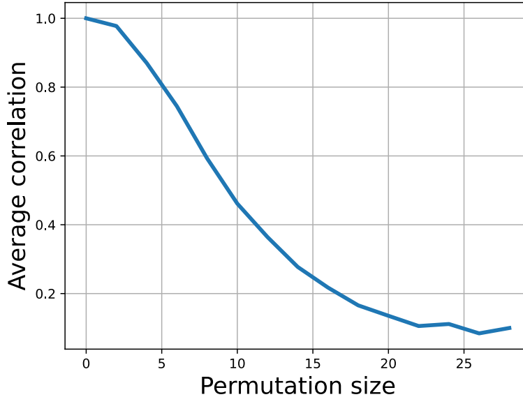
Figure 8: Results of the permuted MNIST NTK feature similarity experiment.
