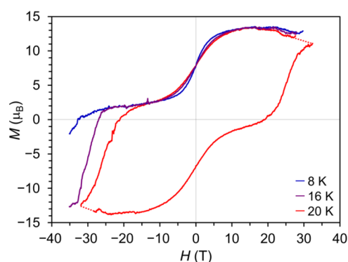
Figure 4. Variable-field magnetization data obtained for 1-Ho between \pm 35 \text{ T} at 20 K (red) overlaid with field-cooled magnetization data collected at 16 K (purple) and 8 K (blue), as described in the text. All data were collected using a sweep rate of 1.7 kOe/s. The dotted lines in the 20 K data are guides for the eye; the measured values in these regions showed an anomalous jump (see Figure S25), which is an artifact likely due to sample movement at such high fields.
