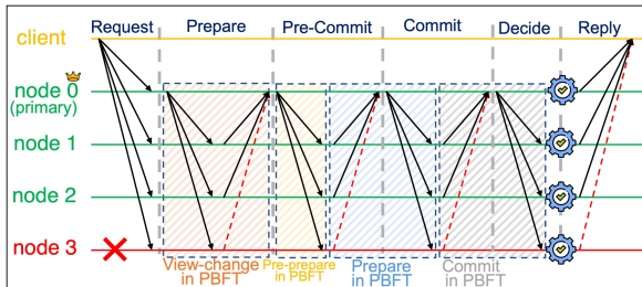
Figure 15: HotStuff
