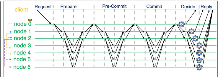
Figure 16: Kauri
