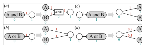
Figure 8: Node breakdown and graph transformation for describing logic relations. (a) and (b) describe the graph transformation for the condition event involving logic relations ( AND and OR ); (c) and (d) are for converting the consequent operation with logic relations.
