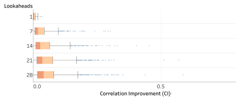
(g) CI for SafeGraph Inflows Mobility
