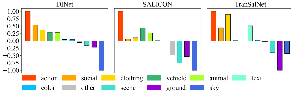
Figure 4: Semantic weights for different saliency models.
