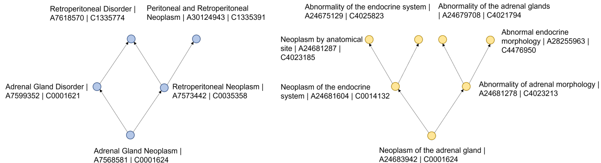
Figure 1: Ancestor subgraphs obtained for two atoms: “Adrenal Gland Neoplasm” from NCIt (left) and “Neoplasm of the adrenal gland” from HPO (right).
