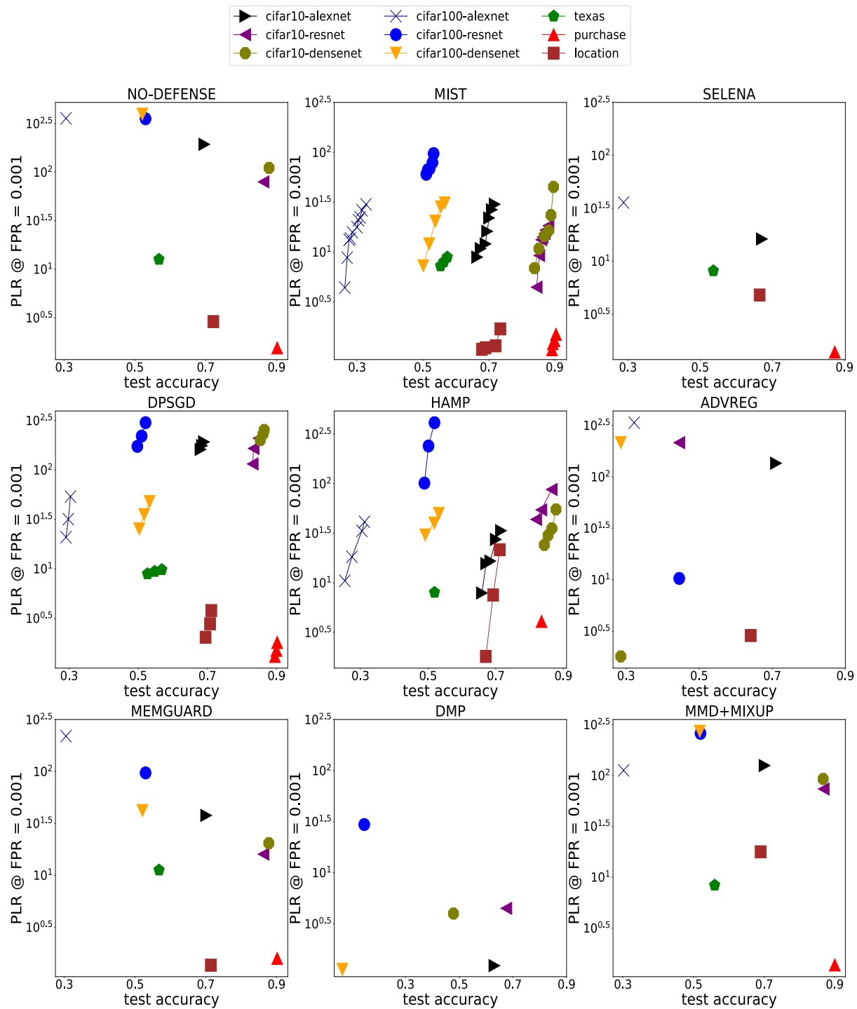
Figure 5: Comparing all defenses using the highest MI attack PLR @ 0.001 FPR among all evaluated attacks. We show the results for each defense in one sub-figure. Notice that for PURCHASE, TEXAS and LOCATION datasets the mixup data augmentation is not applied.
