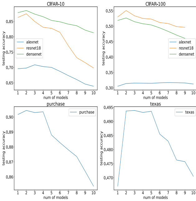
Figure 6: Testing accuracy v.s. number of models for all datasets and models considered in this paper. No mixup data augmentation. The main observation is that testing accuracy can be improved by adding a few models. However, adding too many models would cost testing accuracy.
