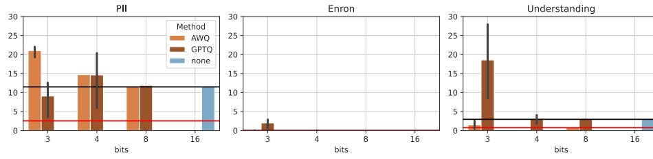
Figure 20. Privacy breakdown scores on LLAMA2 13b Chat.
