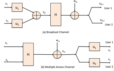
Fig. 2: BC-MAC duality [19]
