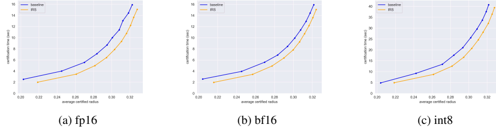
Figure 8: ResNet-20 on CIFAR10 with \sigma = 0.25 .
