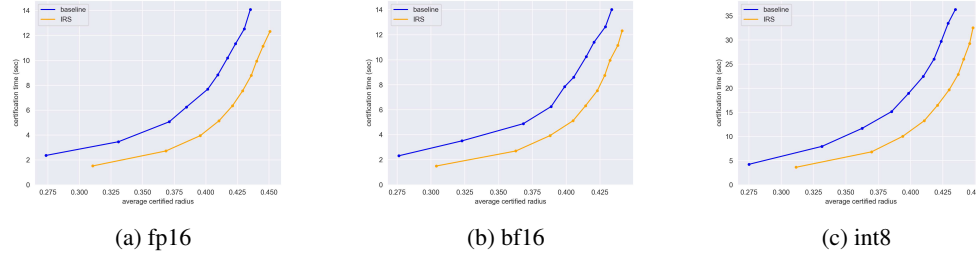
Figure 9: ResNet-20 on CIFAR10 with \sigma = 0.5 .
