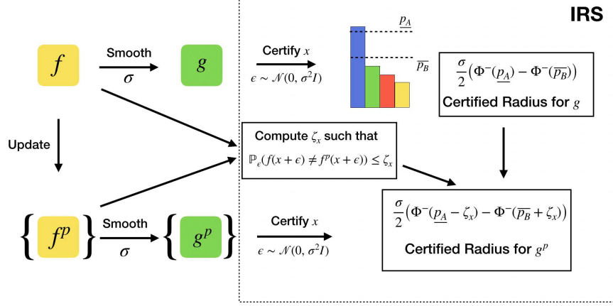
Figure 1: Workflow of IRS from left to right. IRS takes the classifier f and input x . IRS reuses the \underline{p}_A and \bar{p}_B estimates computed for f on x by RS. IRS estimate \zeta_x from f and f^p . For the smoothed classifier g^p obtained from any of the approximate classifiers f^p it computes the certified radius by combining \underline{p}_A and \bar{p}_B with \zeta_x .
