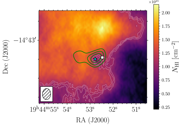
Figure 9. A high-resolution HI column density image measured over the -55 \text{ km s}^{-1} < v_{\text{LSRK}} < -35 \text{ km s}^{-1} in the optically-thin approximation showing the region around the sightline towards NVSS 194452-144311 (cyan star), with the beam shown in the lower corner. Overlaid in green are contours from the convolved \text{H}_2 column density image (see text for details). The faint white contours represent HI column density levels at [1.0, 1.05, \text{ and } 1.1] \times 10^{21} \text{ cm}^{-2} , while the green \text{H}_2 column density contours are at levels of [1.0, 2.0, \text{ and } 3.0] \times 10^{22} \text{ cm}^{-2} . The white square marks the location of the spectrum with the HISA feature shown in the left panel of figure 8.
