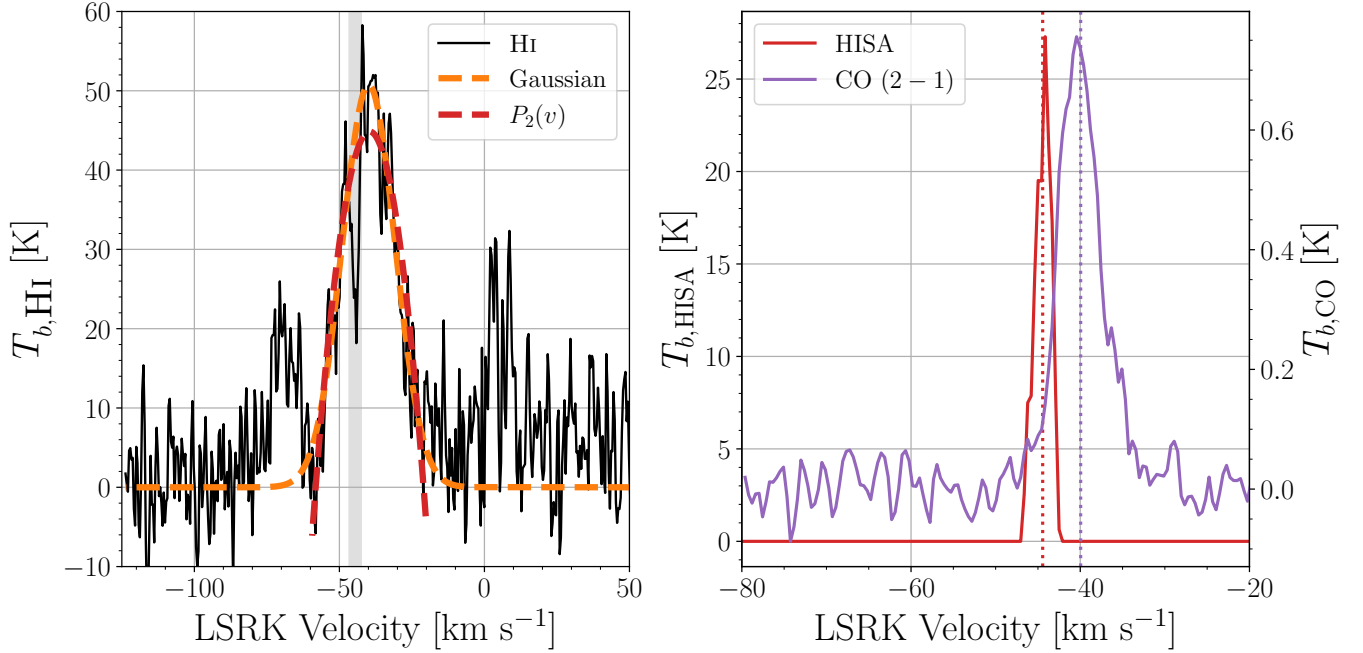
Figure 8. Left: The HI spectrum extracted at \alpha_{\text{J2000}}=19^{\text{h}}44^{\text{m}}52.47^{\text{s}}, \delta_{\text{J2000}}=-14^{\circ}43'10.90'' ( T_{\text{on}} ). The narrow dip centered near -45 \text{ km s}^{-1} results from a potential HISA feature. The orange and red dashed lines respectively represent fits from Gaussian and second-order polynomial functions over the HI emission feature spanning from -60 \text{ km s}^{-1} to -20 \text{ km s}^{-1} with velocities from -42.5 \text{ km s}^{-1} to -47 \text{ km s}^{-1} excluded, as highlighted by the grey shaded region, to model an off spectrum ( T_{\text{off}} ). Right: The HISA spectrum ( T_{\text{off}} - T_{\text{on}} ), depicted in red (brightness temperature on the left y-axis), compared with a spatially-matched CO (2 – 1) spectrum (brightness temperature shown on the right y-axis). Vertical dashed lines denote the respective intensity-weighted velocity centroids.
