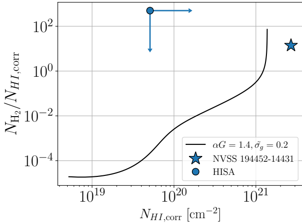
Figure 10. The observed N_{\text{H}_2} -to- N_{\text{HI,corr}} ratio (blue star) compared with predictions from an analytical model developed in the analytical and numerical works of Krumholz et al. 2008, 2009b; McKee & Krumholz 2010; Sternberg et al. 2014; Bialy & Sternberg 2016. Specifically, see the procedure outlined in the introduction of Section 3 Bialy & Sternberg (2016). The black curve represents the model prediction with two observationally-constrained input parameters (see text). The error bars for the observed N_{\text{H}_2} -to- N_{\text{HI,corr}} ratio are shown but are too small to see.
