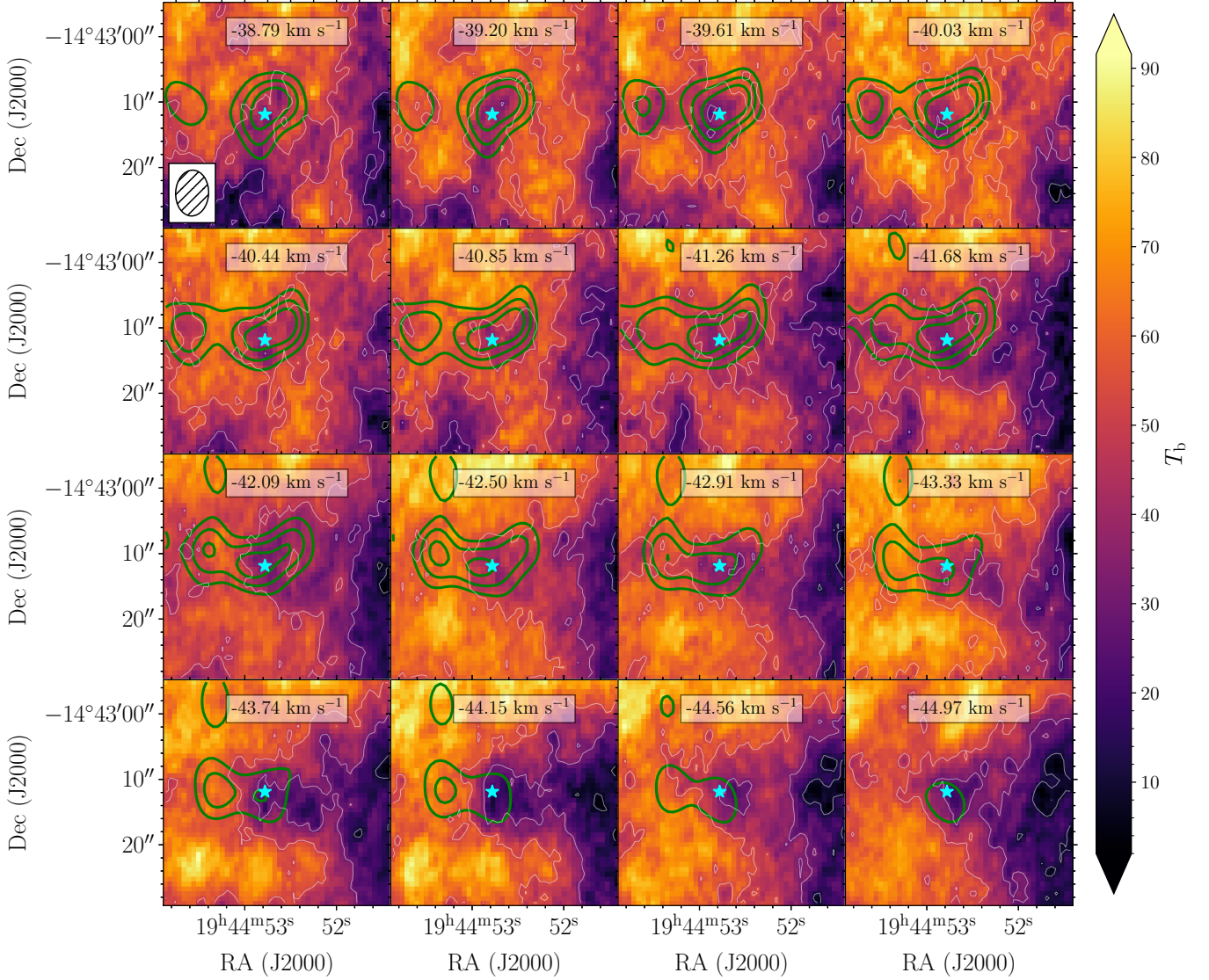
Figure 7. Select channel maps of the high-resolution HI emission (background image and white contours) with contours from CO (2–1) emission (green) smoothed to the resolution of the HI emission data and the location of the sightline towards NVSS 194452-144311 (cyan star) overlaid. The contours representing HI emission are at levels of 10 K, 30 K, and 50 K, while the CO (2–1) emission contours are at levels of 0.25 K, 0.5 K, and 0.75 K.
