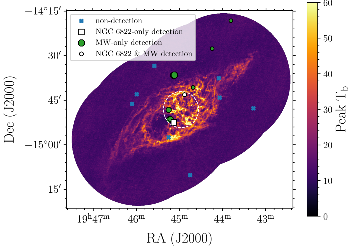
Figure 1. The peak H I brightness temperature image of NGC 6822 from LGLBS. This image does not contain single dish observations to correct for the missing short spacings. The locations of background sources used in our search for absorption are denoted by the overlaid symbols. The different shapes classify our detections: non-detections (blue cross), absorption only at velocities corresponding to Milky Way foreground (green octagons), absorption at velocities corresponding to Milky Way foreground and NGC 6822 (white circle), and absorption only reliably detected at the velocities of NGC 6822 (white square). The symbol sizes indicate the relative flux density level of the background source. The two white symbols show the location of H I absorption at the LSR velocities of NGC 6822 and are highlighted in the profiles shown in Figure 3. The dashed white circle shows the mean radius of the H I column density of 6 \times 10^{20} \text{ cm}^{-2} .
