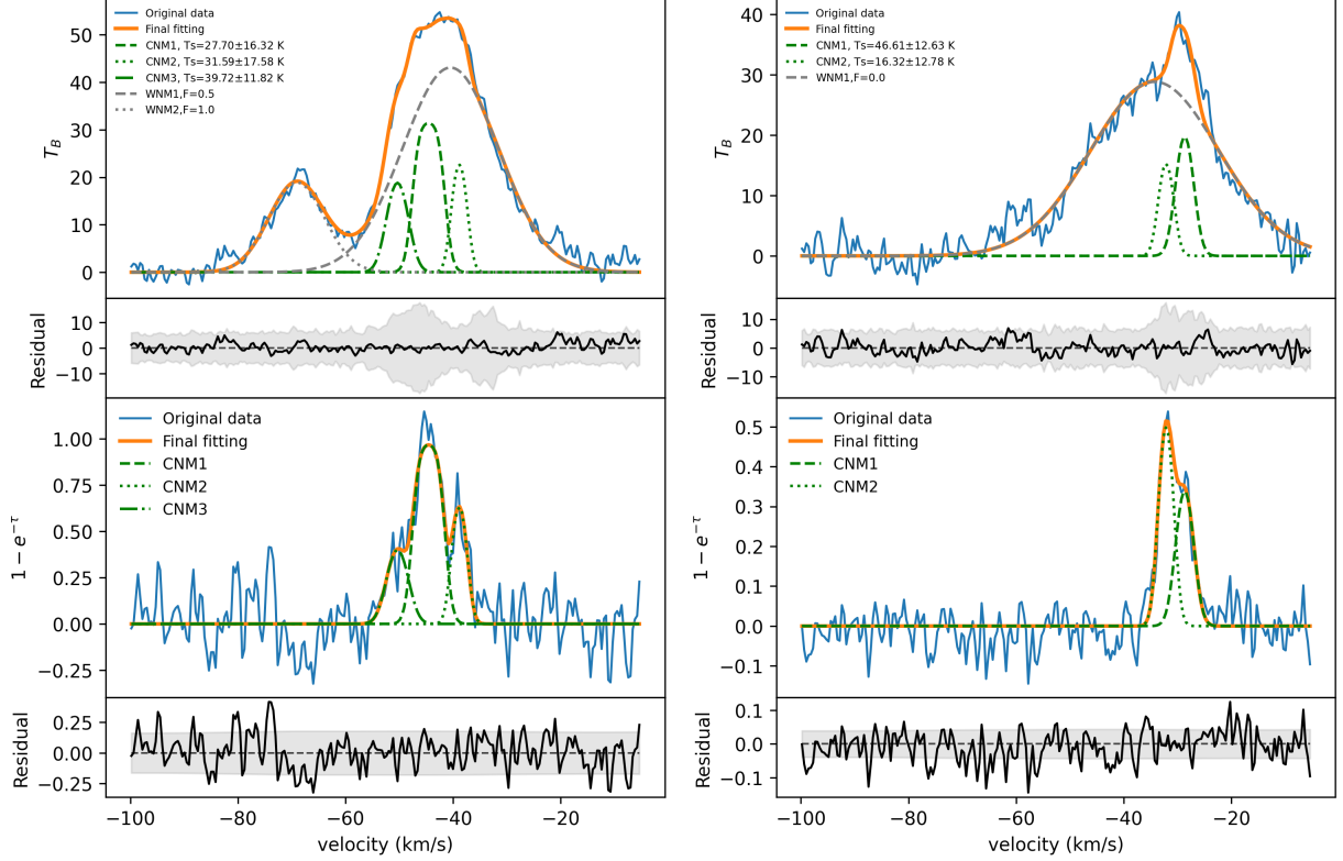
Figure 5. Gaussian decomposition for two absorption-detected sources. The left is source NVSS J194452-144311 and the right source is NVSS J194507-145233. The top two panels show the H I brightness temperature and its corresponding fitting residuals. The bottom two panels present the H I optical depth and its fitting residuals. The top panel specifies the weighted mean spin temperature of the CNM. The ‘F’ value following each ‘WNM’ label quantifies the fraction of the WNM absorbed by the CNM, as stated in the text. The gray shaded area in the residual indicates the 1\sigma error of the emission/absorption spectra.
