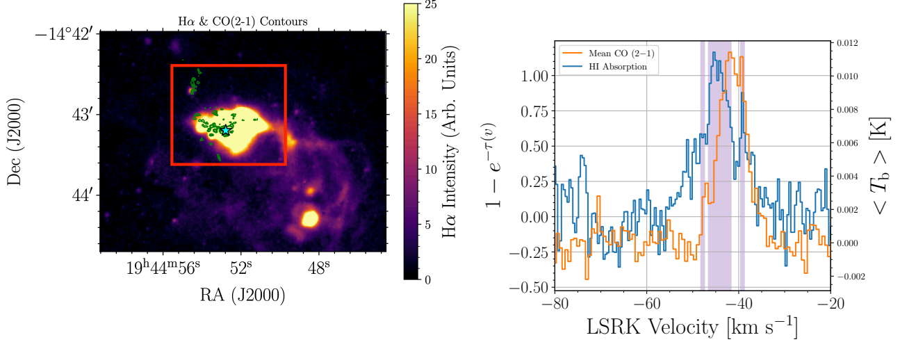
Figure 6. Left: Map of the H \alpha intensity from Hunter & Elmegreen (2004) with the location of the northern HI absorption (cyan star) and contours of CO (2–1) observations from Schrubba et al. (2017) at levels of 5, 10, and 15 K km s −1 overlaid. Right: the HI absorption spectra (blue) compared with a mean brightness temperature spectrum of CO (2–1) (orange) measured within the red box overplotted on the H \alpha map. The purple shaded regions represent spectral channels with absorption signal exceeding the 3 \sigma level. The left y-axis shows units of optical depth, while the right y-axis shows the mean brightness temperature of the CO.
