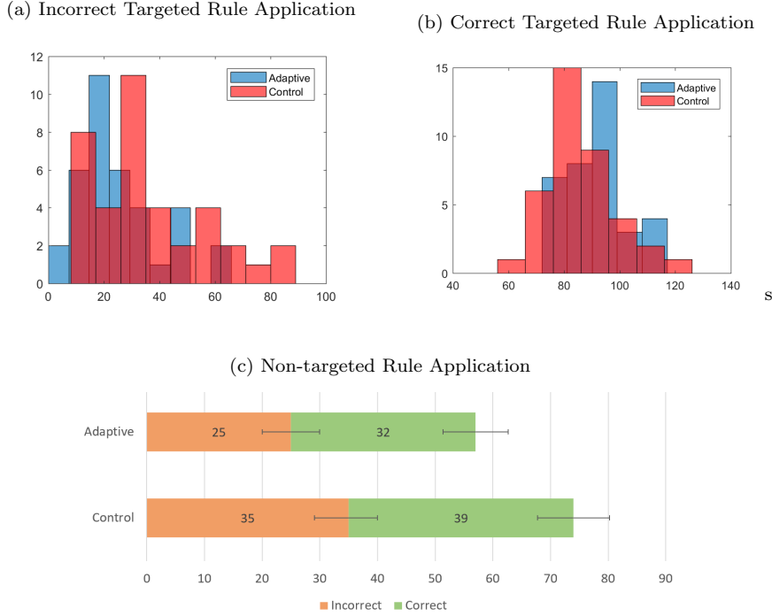
Fig. 3: The HNU Adaptive has significantly fewer incorrect targeted rule applications ( p = .02 ), and significantly more correct targeted rule applications ( p = .02 ) than HNU Control. And, there are no significant differences in non-targeted correct and incorrect rule applications between the two groups
