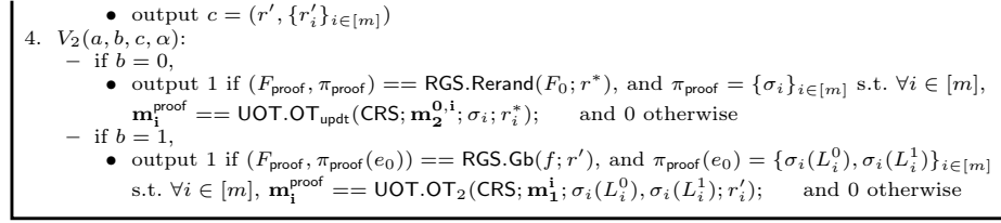
Fig. 14 \Sigma -protocol for Correct Garbling
