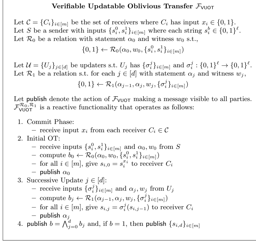
Fig. 10 Verifiable Updatable Oblivious Transfer
