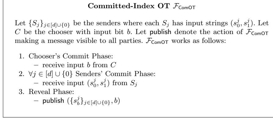
Fig. 18 Committed-Index OT
