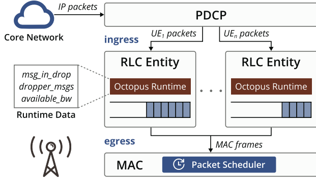
Figure 5: Base-station (eNB/gNB) protocol stack with Octopus
