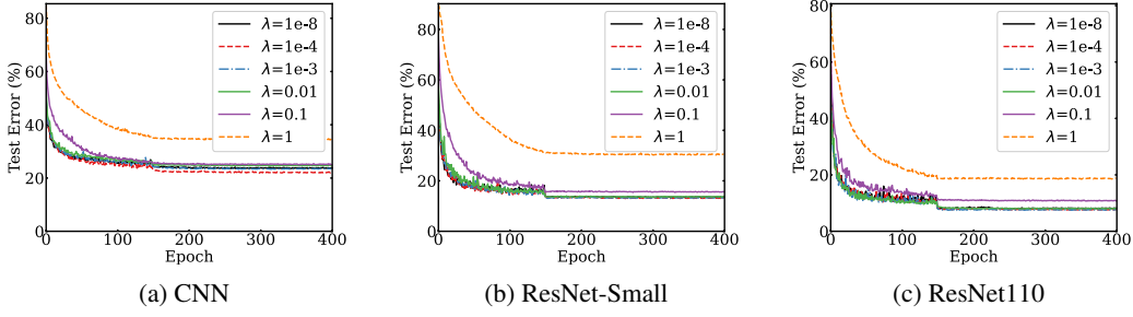
Figure 1: Test errors of different models trained on CIFAR-10 using the Adam optimizer with \beta = 0.9, \beta_{sq} = 0.999, \eta = 0.001 and different \lambda s. From left to right: (a) a shallow CNN with 6 layers; (b) ResNet-Small with 20 layers; and (c) ResNet110 with 110 layers.
