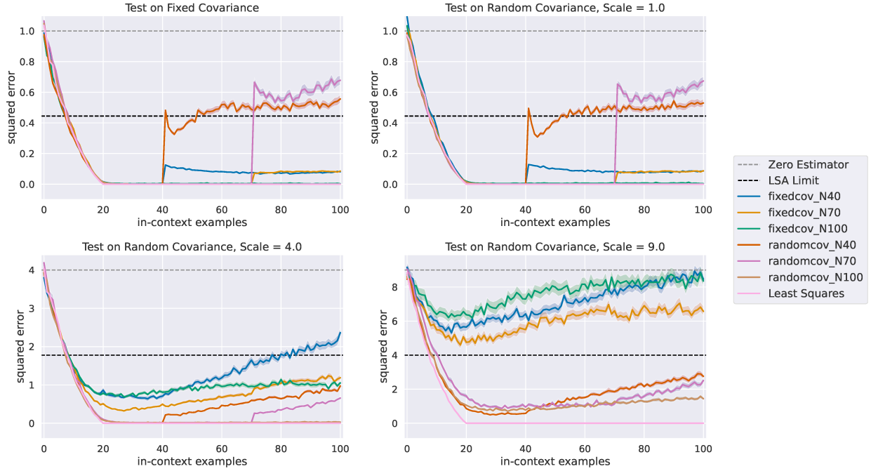
Figure 1: Normalized prediction error for transformers with GPT2 architectures as a function of the number of in-context test examples M when trained on in-context examples of linear models in d = 20 dimensions. Colored lines correspond to different training context lengths ( N \in \{40, 70, 100\} ) and different training procedures (either a fixed identity covariance matrix or random diagonal covariance matrices with each diagonal element sampled i.i.d. from the standard exponential distribution). The four figures correspond to evaluating on either fixed covariance or random covariance matrices of different scales. The gray dashed line shows the prediction error of zero estimator and the black dashed line the prediction error of LSA model when M, N \rightarrow \infty . The GPT2 models achieve smaller error when they are trained on random covariance matrices with larger contexts, but their prediction error spikes when evaluated on contexts larger than those they were trained on.
