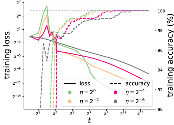
Figure 2: Training loss and training accuracy of (GD) for logistic regression on a subset of MNIST. This is a replication of Figure 1 with training accuracy curves. The plots show that the stable phase is entered before reaching 100% training accuracy. Moreover, GD with larger stepsizes reaches perfect training accuracy faster.
