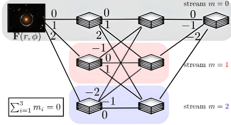
Figure 1: Example of a Harmonic Network with two hidden layers. Each horizontal stream represents a series of feature maps of constant rotation order, while the edges represents cross-correlations.
