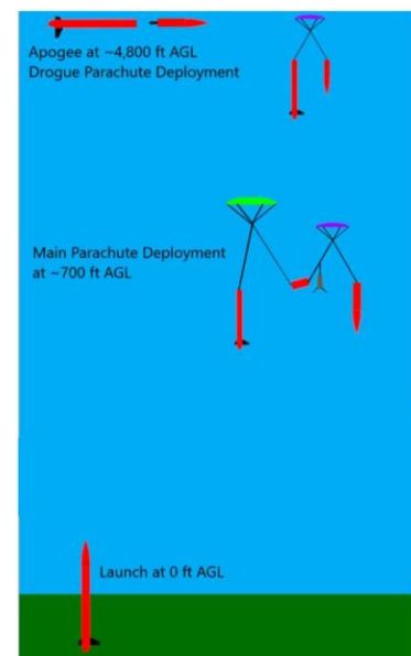
Figure A1: STAGES OF FLIGHT OF PARACHUTE AND PAYLOAD
