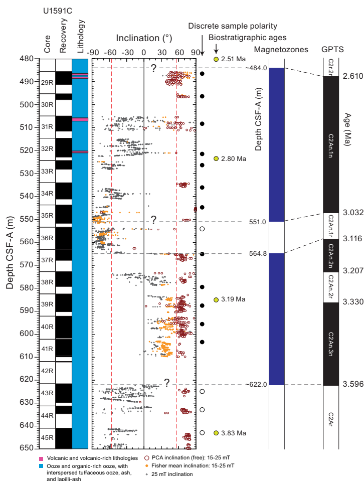
Figure F39. Archive-half section magnetic inclinations for 480–650 mbsf, Hole U1591C. Data are used to define magnetozones that are correlated to the geomagnetic polarity timescale (GPTS) of Gradstein et al. (2020). Red dashed lines = geocentric axial dipole inclinations expected at this site. Solid/open circles = normal/reversed polarity of discrete samples.
