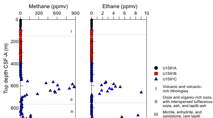
Figure F52. Headspace gas analyses of methane, Site U1591. Dashed lines = unit boundaries.
