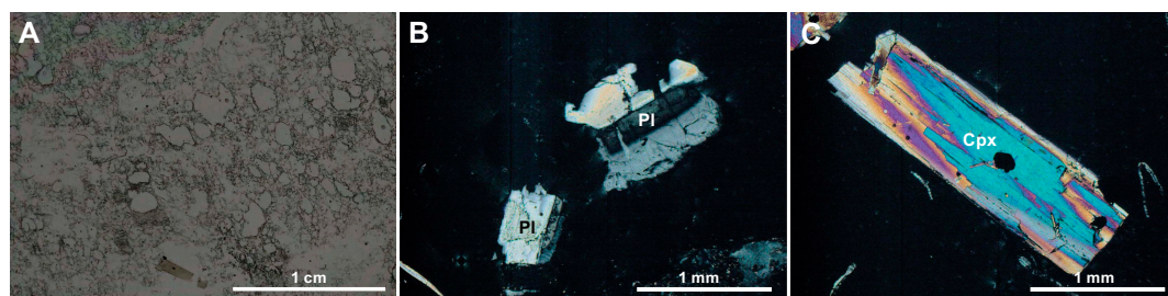
Figure F9. Light-colored, highly vesicular, porphyritic pumice from Unit I, Hole U1591A (9H-2, 70–73 cm). A. Vesicle-rich and crystal-poor nature of the pumice (plane-polarized light [PPL]). Phenocrysts of (B) plagioclase (Pl) and (C) clinopyroxene (Cpx), which occur together with Fe-Ti oxide (cross-polarized light [XPL]). Rare apatite occurs as inclusions in pyroxene. The glassy groundmass shows patchy alteration.
