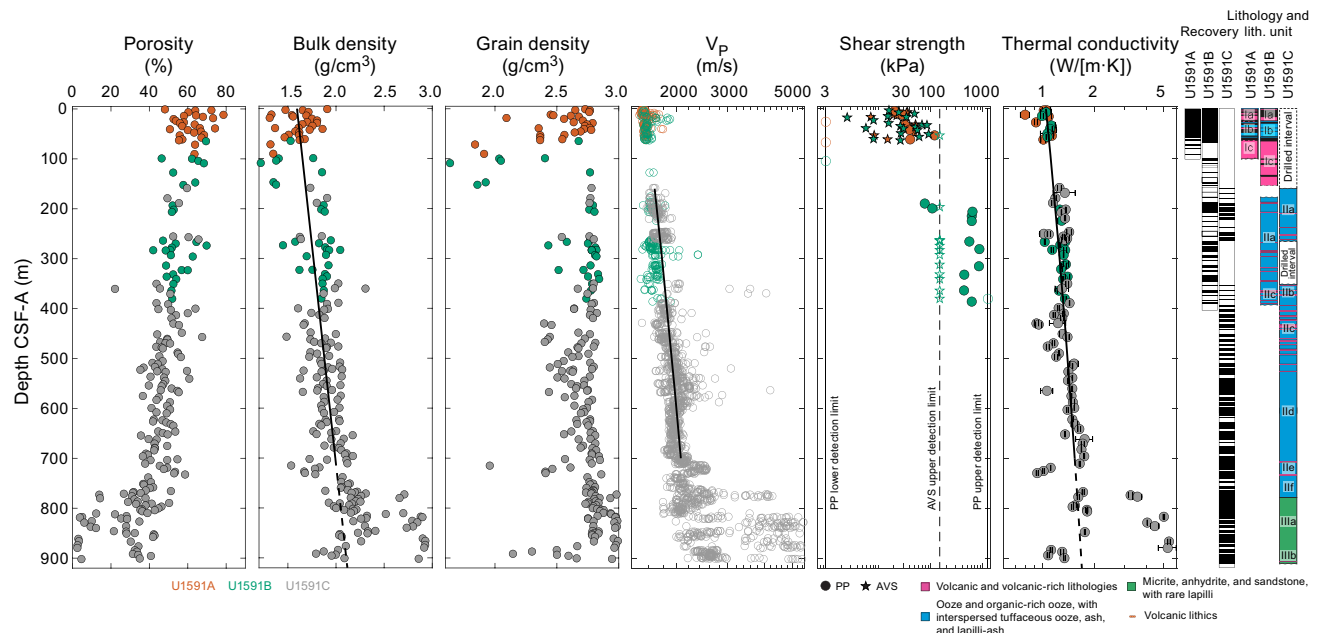
Figure F46. Discrete physical property measurements, Site U1591. Sediment below shear strength measurements shown was too stiff for measurement. Solid curves = linear least-squares best fits to the data, dashed lines = extrapolations.
