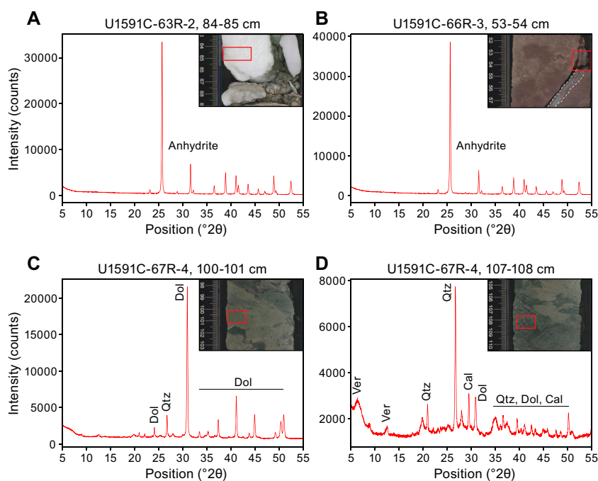
Figure F18. Selected XRD spectra of Unit III evaporite lithologies, Hole U1591C. A. Massive anhydrite. B. Anhydrite veinlet. C. Interval dominated by dolomite with minor quartz. D. Interval characterized by a multimineral assemblage of dolomite and quartz with minor calcite and vermiculite. Qtz = quartz, Dol = dolomite, Ver = vermiculite, Cal = calcite.
