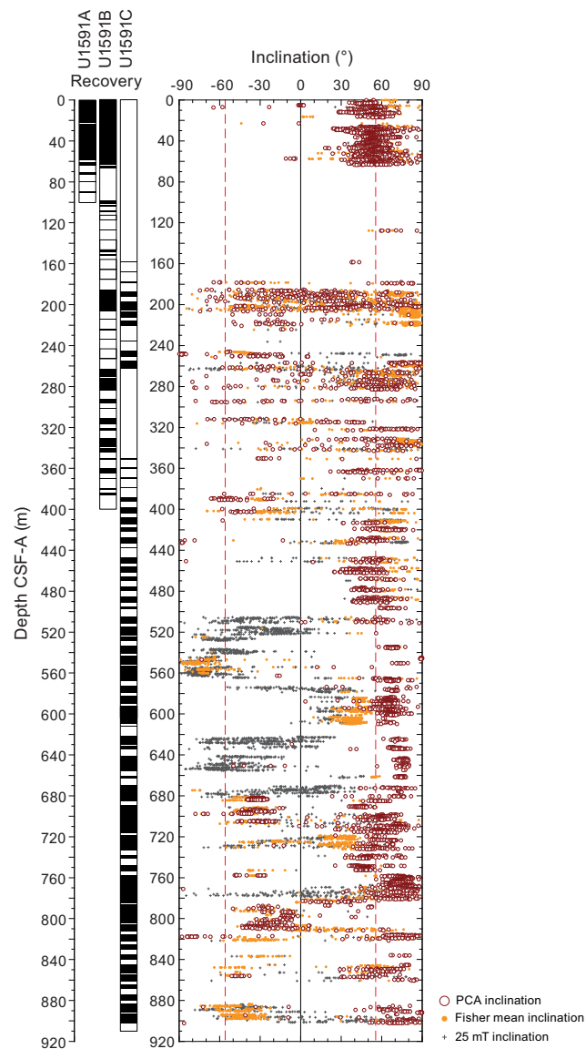
Figure F38. Archive-half section magnetic inclinations, Site U1591. Red dashed lines = geocentric axial dipole inclinations expected at this site.
