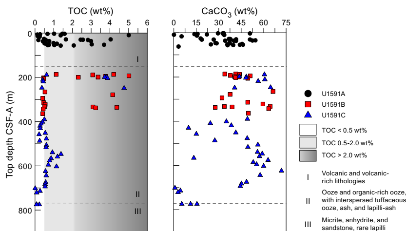
Figure F51. TOC and carbonate, Site U1591. Dashed lines = unit boundaries. Sapropel conventions follow Kidd et al. (1978).
