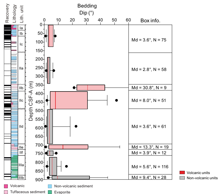
Figure F23. Box plots of bedding dip distribution in lithostratigraphic units, Site U1591. The minimum (P5), first quartile (P25), median value (P50), third quartile (P75), and maximum (P95) are shown. Only the first outlier that is smaller than P5 and larger than P95 is plotted as a dot. Md = median dip, N = number of samples.
