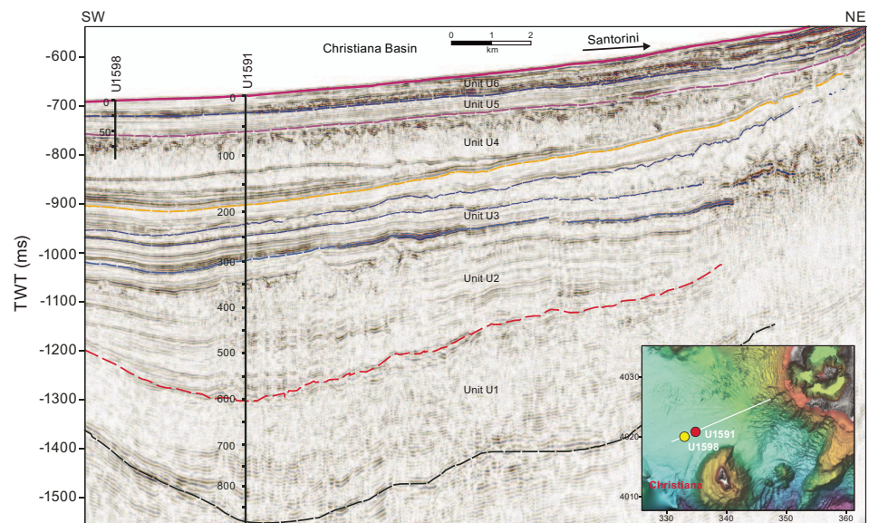
Figure F2. Seismic profile across the Christiana Basin along Seismic Line Geomar_P5008. The basin fill has six seismic stratigraphic units (U1–U6), following Preine et al. (2022b). Inset: locations of Site U1591 and Site U1598 in the same basin. Depths in meters.
