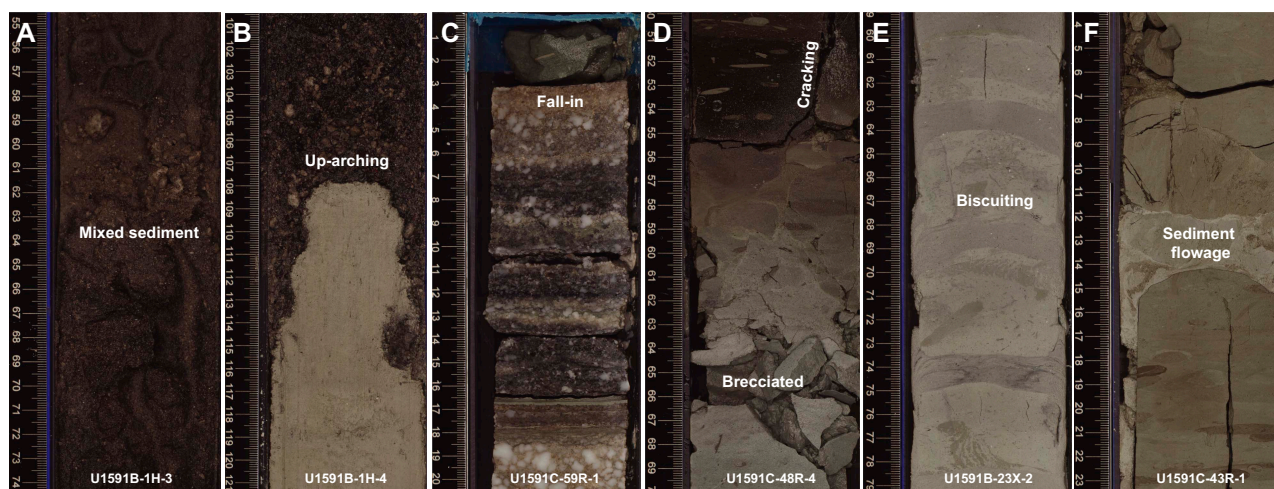
Figure F6. Core disturbances, Site U1591. A. Mixed sediments. B. Uparching. C. Fall-in. D. Cracking and brecciated core. E. Biscuiting. F. Sediment flowage.
