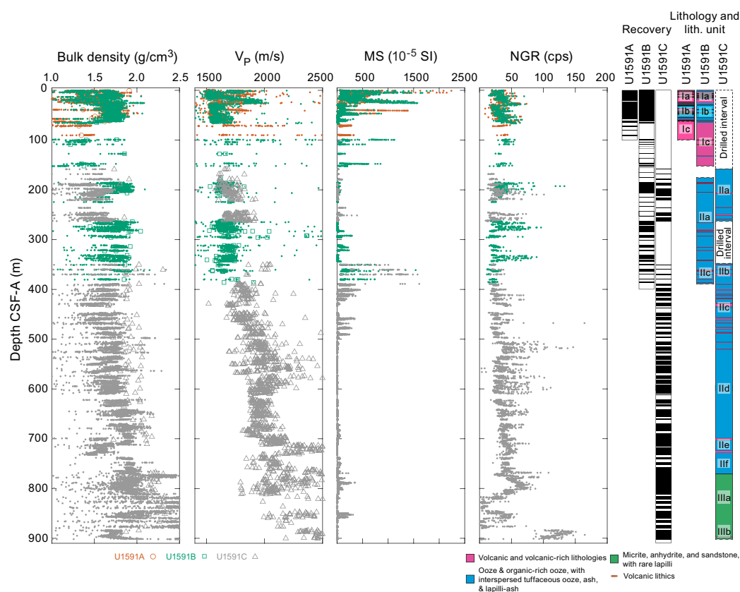
Figure F43. Physical properties, Site U1591. Dots = whole-round measurements, open symbols = discrete sample measurements. Samples with bulk density and P -wave velocity greater than the maximum values on the x-axes are plotted in Figure F46. cps = counts per second.
