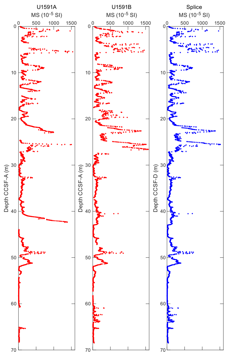
Figure F19. WRMSL-derived MS data, Holes U1591A and U1591B. The spliced section is shown in the right panel. Note that MS data are on the CCSF-A depth scale and the spliced section is on the CCSF-D depth scale. MS data were clipped at 1600 \times 10^{-5} SI.
