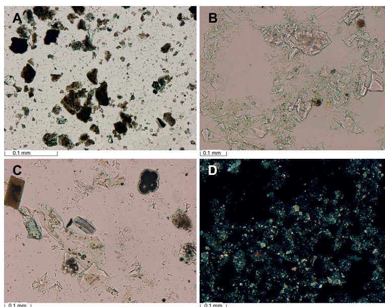
Figure F8. Ooze, Hole U1591A. A. Ooze layer (3H-2). B. Ooze with mud (2H-2). C. Ooze with ash (8H-1). D. Tuffaceous mud (8H-2).
