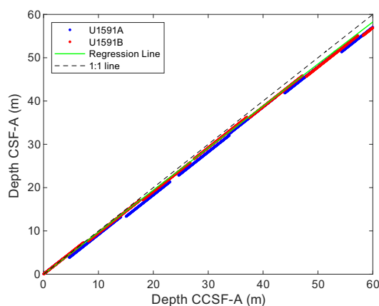
Figure F21. CCSF-A versus CSF-A core depths, Holes U1591A and U1591B. Lines fit through the core depths of all holes give an estimate of the affine growth factor. At Site U1591, this is estimated to be approximately 3%.
