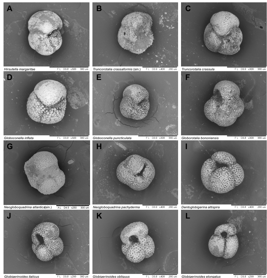
Figure F31. Planktonic foraminifera, Site U1591. A. Hirsutella margaritae . B. Truncorotalia crassaformis (sinistral) (398-U1591C-20R-CC, 10–15 cm). C. Truncorotalia crassula (398-U1591B-32X-CC, 37–40 cm). D. Globoconella inflata (1H-CC, 20–23 cm). E. Globoconella puncticulata . F. Globorotalia bononiensis (398-U1591C-31R-CC, 19–21 cm). G. Neogloboquadrina atlantica (sinistral) (398-U1591B-42X-CC, 0–3 cm). H. Neogloboquadrina pachyderma (398-U1591A-7H-CC, 24–27 cm). I. Dentoglobigerina altispira . J. Globigerinoides italicus (398-U1591C-48R-CC, 0–4 cm). K. Globigerinoides obliquus (56R-CC, 8–10 cm). L. Globigerinoides elongatus . (A, L: 47R-CC, 0–2 cm; E, I: 45R-CC, 23–25 cm).
