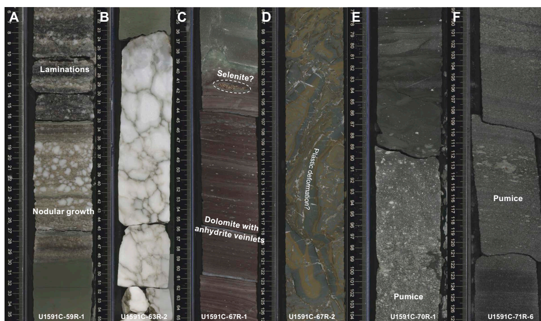
Figure F14. Representative lithologies from Unit III, Hole U1591C. A, B. Laminated and nodular anhydrite. C. Dolomite with anhydrite veinlets. D. Anhydrite with evidence of plastic deformation and secondary mineralization. E, F. Pumice lapilli within anhydritic mudstone and micrite. A–D: Subunit IIIa; E–F: Subunit IIIb.
