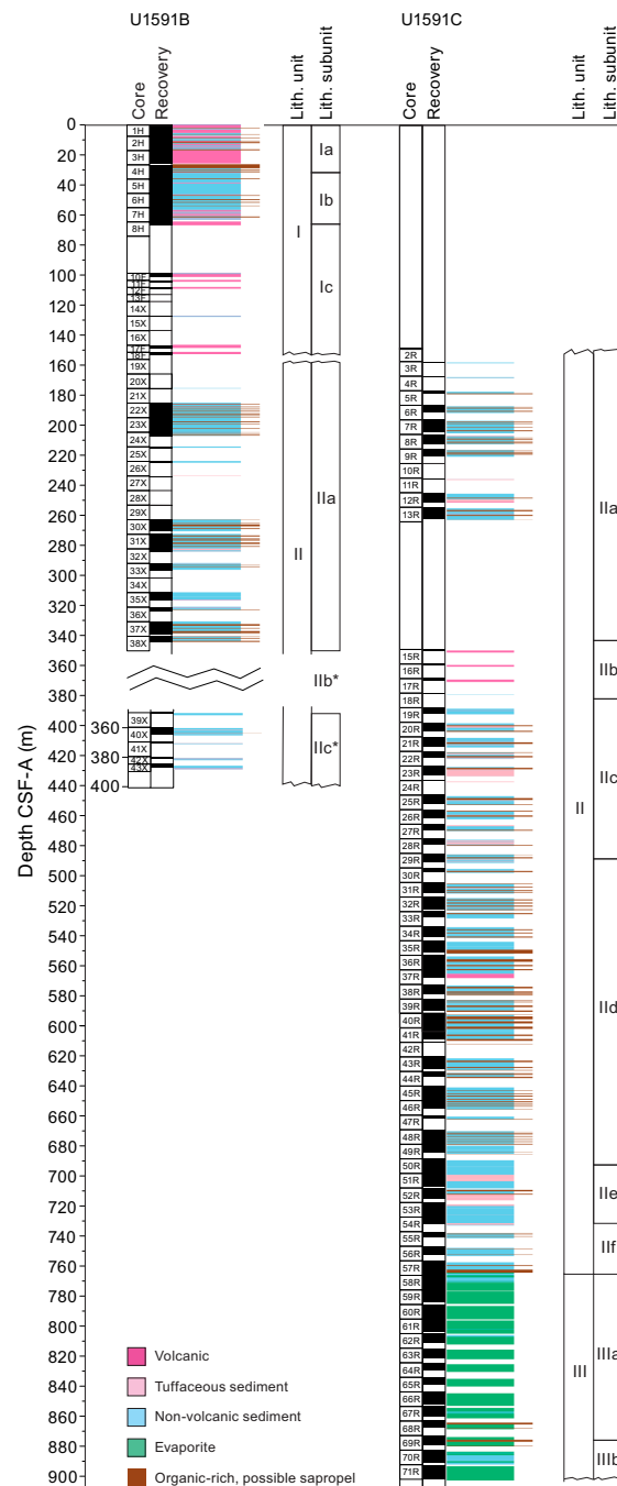
Figure F11. Organic-rich, sapropelic lithologies (extended brown lines), with background lithologies, Holes U1591B and U1591C. Confirmation of sapropelic units requires geochemical analysis of TOC content (see Geochemistry). Gaps in lithologies indicate gaps in recovery, as shown in Figure F3. * = depth and recovery affected by slumped material.
