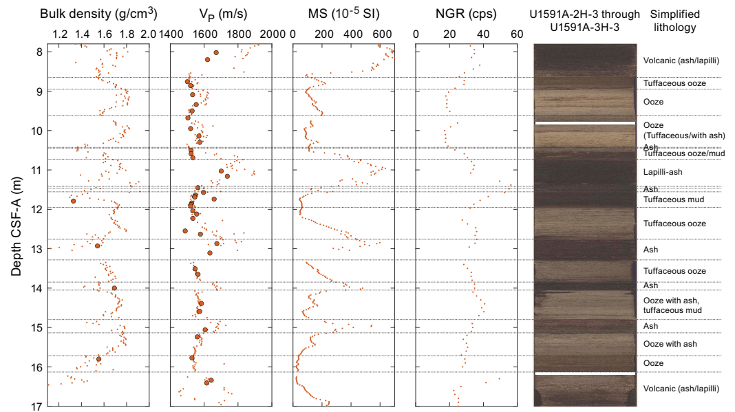
Figure F44. Relationships between lithology and physical properties, Hole U1591A. The top and bottom NGR measurements are removed from each section because the values are affected by edges of sections. White bars on image = void space where IW samples were collected. cps = counts per second.
