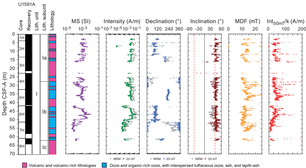
Figure F35. Archive-half section magnetic data, Hole U1591A. Red dashed lines = geocentric axial dipole inclinations expected at this site.
