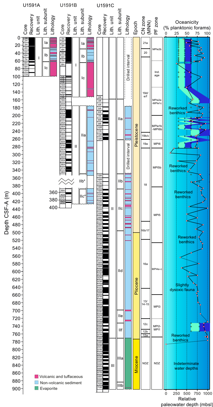
Figure F30. Biostratigraphic summary, Site U1591. CN = calcareous nannofossil, MNN = Mediterranean Neogene Nannoplankton, PF = planktonic foraminifer. Interpreted oceanicity (Hayward et al., 1999): solid line/red points = interpreted oceanicity, dashed line = extrapolation through barren/unreliable sample data. Interpreted paleowater depths: light blue points/shading = shallower paleowater depth interpretation, dark blue points/shading = deeper paleowater depth interpretation. * = depth and recovery affected by slumped material.
