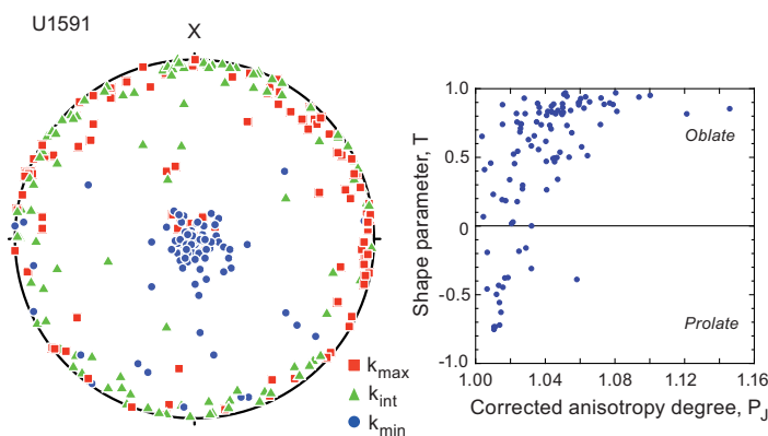
Figure F42. Discrete sample anisotropy of low-field magnetic anisotropy, Hole U1591C. Left: lower hemisphere stereographic equal-area projections of principal anisotropy axes (min = minimum, int = intermediate, max = maximum). Right: shape parameter plotted against corrected anisotropy degree (Jelinek and Kropáček, 1978).
