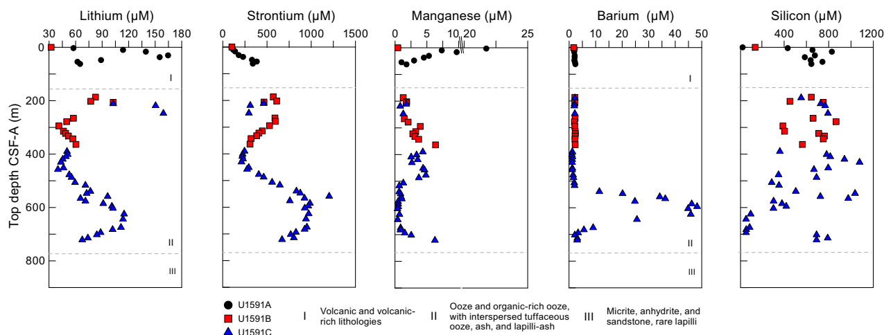
Figure F50. ICP-AES concentrations of Li, Sr, Mn, Ba, and Si in IW samples, Site U1591. Dashed lines = unit boundaries.
