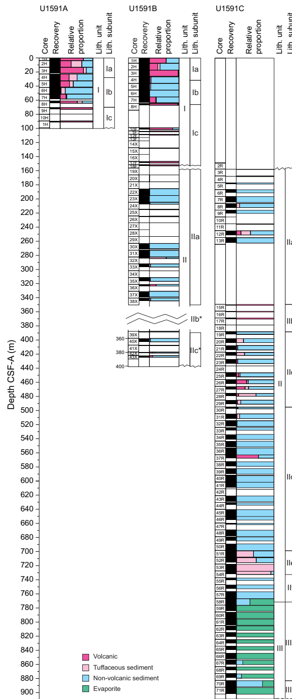
Figure F4. Relative percentages of volcanic, tuffaceous, and nonvolcanic lithologies, Site U1591. Unit I is volcanic rich compared to the nonvolcanic-dominated Unit II. Unit I subunits correspond to smaller scale variations of volcanic vs. nonvolcanic lithologies. * = depth and recovery affected by slumped material.
