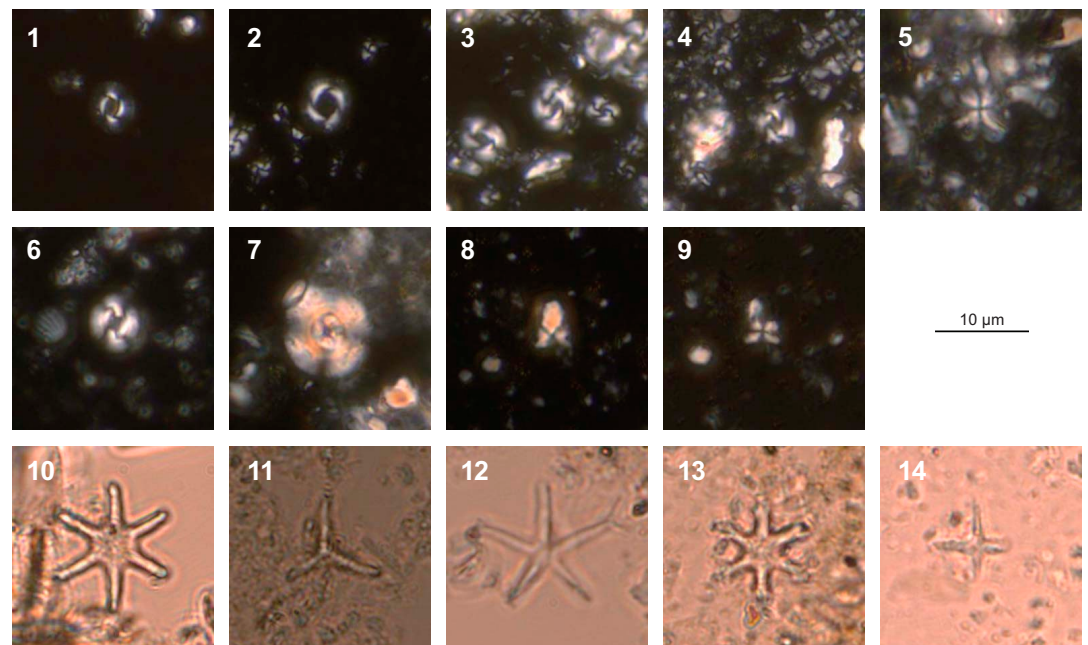
Figure F28. Calcareous nannofossils. 1. Emiliana huxleyi (Lohmann) Hay and Mohler (398-U1591A-3H-CC, 17–20 cm). 2. Pseudoemiliana lacunosa (Kamptner) Gartner, (8H-1, 39–41 cm). 3, 4. 398-U1591B-24X-CC, 38–41 cm: (3) Gephyrocapsa spp. large form (>5.5 µm); (4) Gephyrocapsa oceanica Kamptner. 5. Sphenolithus abies Deflandre (398-U1591C-48R-CC, 0–4 cm). 6. Reticulofenestra pseudoumbilicus (Gartner) (54R-CC, 42–49 cm). 7. Cyclicargolithus floridanus (Roth and Hay) Bukry (60R-1, 3 cm). 8, 9. Sphenolithus heteromorphus Deflandre (68R-4, 83–86 cm). 10. Discoaster brouweri Tan Sin Hok (23R-CC, 21–24 cm). 11. Discoaster triradiatus Tan Sin Hok (398-U1591B-34X-CC, 0–2 cm). 12. Discoaster pentaradiatus Tan Sin Hok (398-U1591C-29R-CC, 0–2 cm). 13. Discoaster surculus Martini and Bramlette (31R-CC, 19–21 cm). 14. Discoaster tamalis Kamptner (32R-CC, 21–23 cm).
