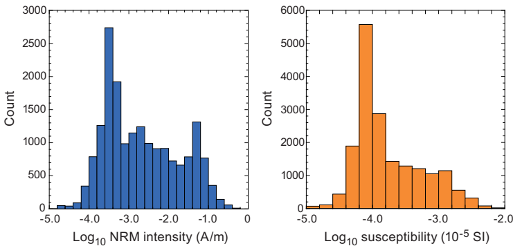
Figure F34. Histograms of NRM intensity and low-field MS, Site U1591. Data are based on archive-half section SRM measurements and low-field point MS measurements made at the same intervals downhole.
