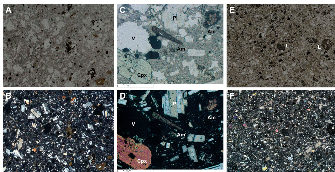
Figure F13. Cobbles in Subunit IIb and sandstone in Subunit IIc, Hole U1591C. A, B. Porphyritic extrusive volcanic rock (17R-1, 49–52 cm). (A) PPL; (B) XPL. C, D. Phenocrysts of plagioclase (Pl), amphibole (Am), clinopyroxene (Cpx), and vesicles (V) in the same sample. (C) PPL; (D) XPL. Other phenocrysts in the sample include orthopyroxene (hypersthene), the dominant pyroxene type, and Fe-Ti oxide (Ti-magnetite). Accessory apatite occurs as inclusions in other phases. Glomerocrysts consist of plagioclase, amphibole, and pyroxene. E, F. Immature sandstone (28R-1, 46–48 cm) with abundant grains of plagioclase, benthic foraminifera, and other bioclasts as well as volcanic lithics (L), typically scoria. (E) PPL; (F) XPL.
