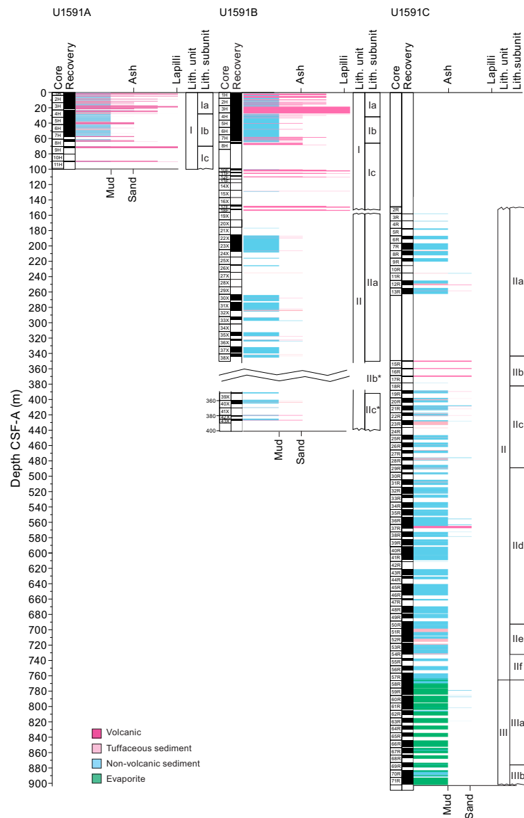
Figure F5. Average grain size distribution of volcanics, Site U1591. Length of colored bars = relative grain sizes (ash = <2 mm; lapilli = 2–64 mm; mud = <63 \mu m; sand = 0.063–2 mm), with separate scales shown for volcanic grain size (top) and tuffaceous and nonvolcanic sediments (bottom). Mixed lithologies such as lapilli-ash that have relative grain sizes between two categories are plotted between ticks. Evaporites (green) are not characterized by grain size. * = depth and recovery affected by slumped material.
