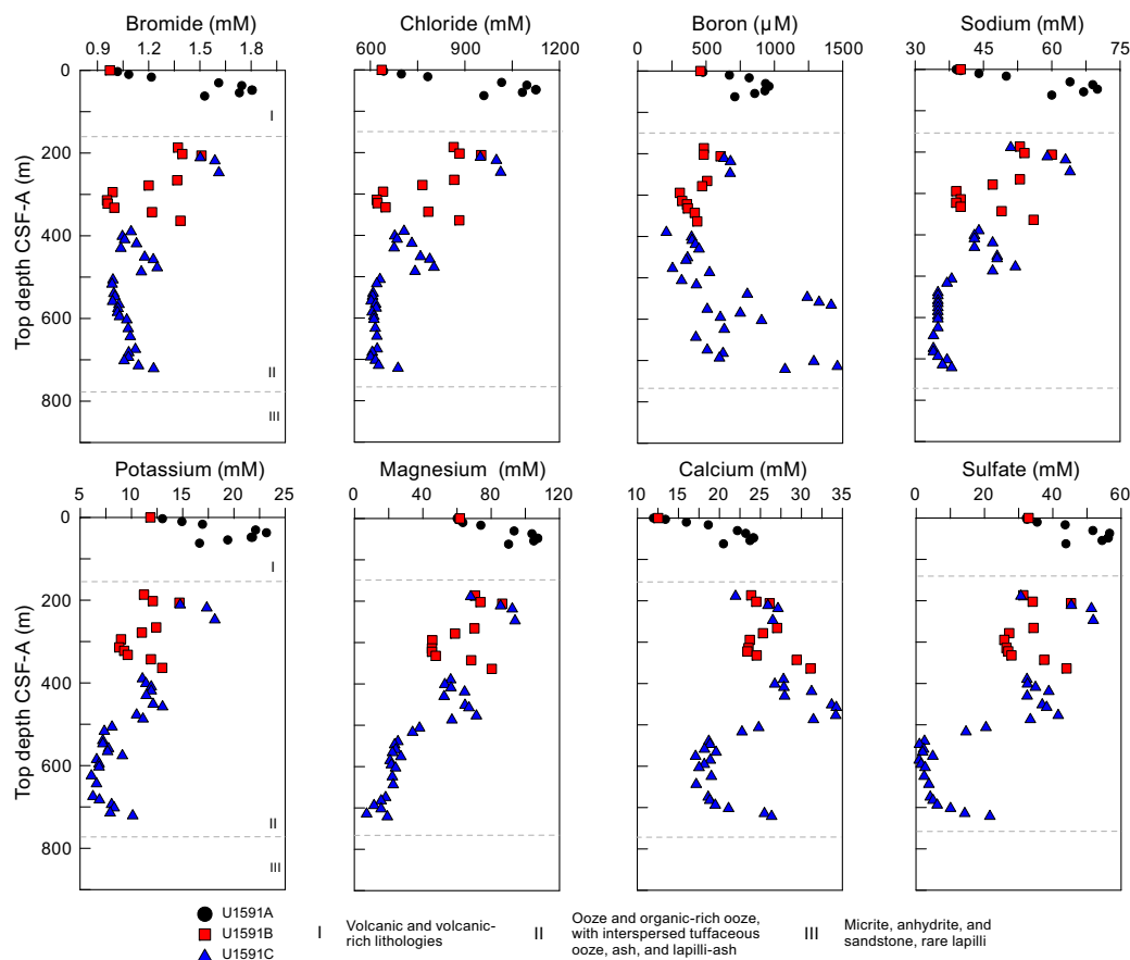
Figure F49. IC and ICP-AES concentrations of Br, Cl, B, Na, K, Mg, Ca, and \text{SO}_4^{2-} in IW samples, Site U1591. Dashed lines = unit boundaries.
