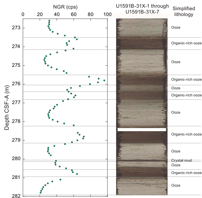
Figure F45. Relationships between NGR and lithology, Hole U1591B. The top and bottom NGR measurements are removed from each section because the values are affected by edges of sections. White bar on images = void space where IW samples were collected. cps = counts per second.
