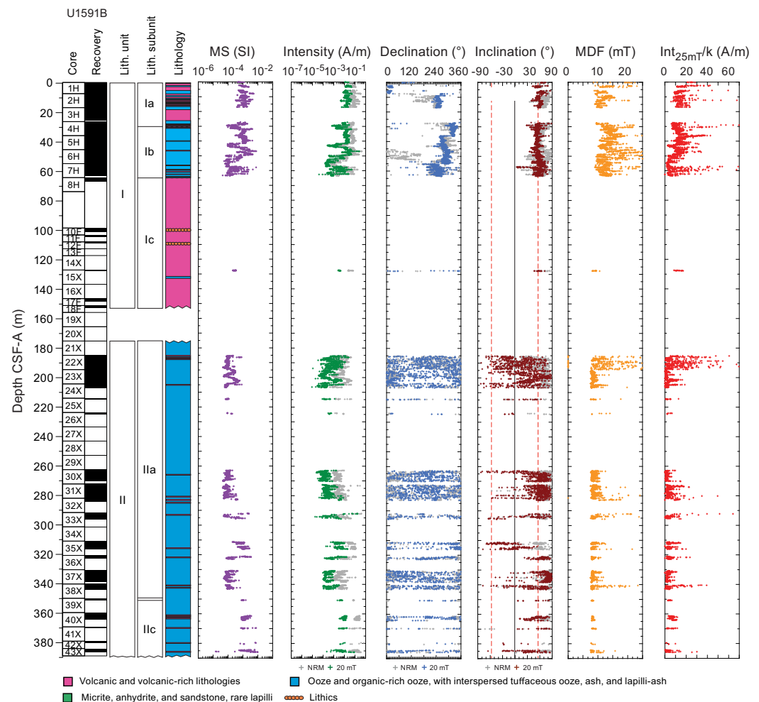
Figure F36. Archive-half section magnetic data, Hole U1591B. Red dashed lines = geocentric axial dipole inclinations expected at this site.
