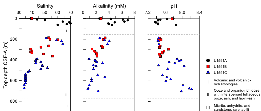
Figure F48. IW salinity, alkalinity, and pH, Site U1591. Dashed lines = unit boundaries.
