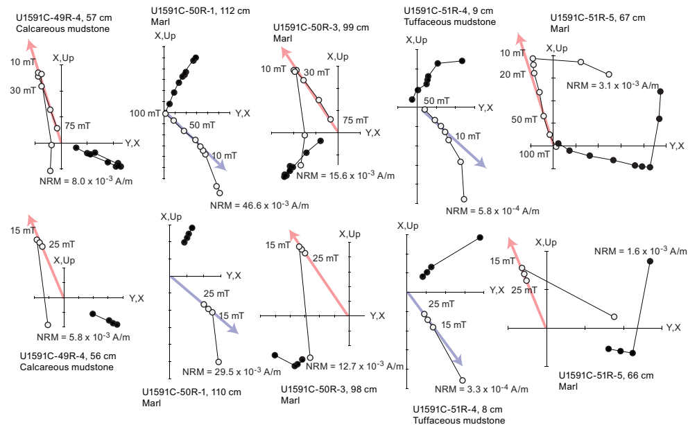
Figure F41. AF demagnetization of discrete samples (top) and archive-half sections (bottom), Site U1591. The series of reversals shown in Figure F40 are documented. Red/blue arrows = reversed/normal polarity inclinations, solid circles = projection onto horizontal plane, open circles = projection onto vertical plane.
