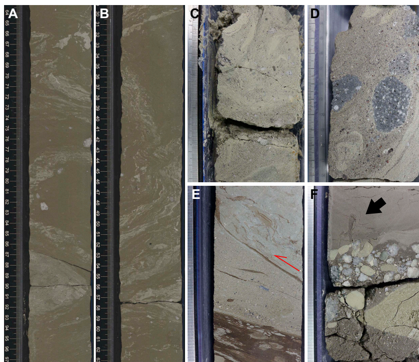
Figure F24. Slumps identified on split core surfaces. A, B. Slump composed of folded sandy laminae/beds in a muddy matrix (398-U1591C-23R-4, 29–97 cm). C. Slump representing block-in-matrix texture containing disturbed/flown muddy clasts within a mud/sand-mixture matrix (398-U1591B-27X-CC, 5–17 cm). D. Slump representing block-in-matrix texture containing pumice and siltstone clasts all within a mud/sand-mixture matrix (398-U1591C-15R-CC, 93–104 cm). E. Base of a slump representing an apparent reverse fault (split arrow; 38R-CC, 37–49 cm). The slip plane is composed of homogenized sand/mud. F. Top of a debris flow deposit (arrow; 398-U1591B-33X-CC, 16–28 cm). Clasts only occur in the uppermost part of the sand layer and indicate reverse grading.
