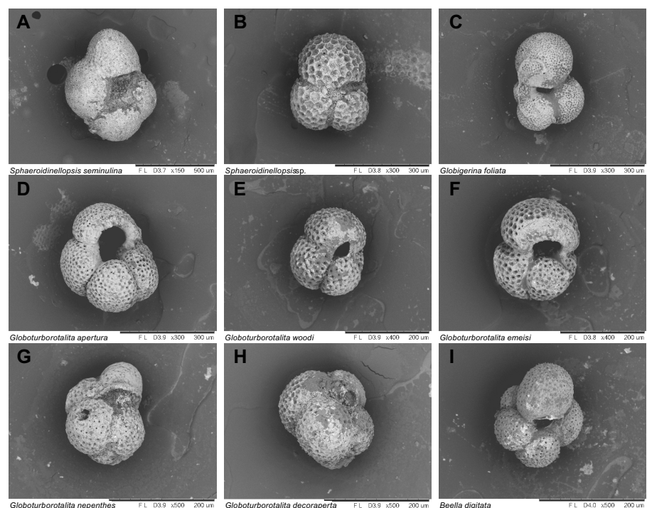
Figure F32. Planktonic foraminifera, Hole U1591C (unless otherwise specified). A. Sphaeroidinellopsis seminulina (56R-CC, 8–10 cm). B. Sphaeroidinellopsis sp. (38R-CC, 67–69 cm). C–F. 47R-CC, 0–2 cm: (C) Globigerina foliata ; (D) Globoturborotalita apertura ; (E) Globoturborotalita woodi ; (F) Globoturborotalita emeisi . G. Globoturborotalita nepenthes (55R-CC, 0–3 cm). H. Globoturborotalita decoraperta (45R-CC, 23–25 cm). I. Beella digitata (398-U1591A-7H-CC, 24–27 cm).
