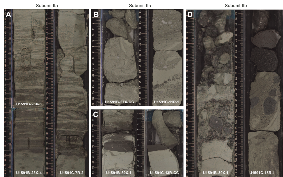
Figure F17. Exemplary correlations between Holes U1591B and U1591C. A. Succession of ooze, strongly bioturbated organic-rich ooze, to ooze. B. Tentatively correlated gravely tuffaceous mud to sand with gravel. Drilling disturbance in this sediment interval was strong in Hole U1591B and slight in Hole U1591C. C. Succession of ooze, organic-rich ooze, to ooze (top to bottom) disturbed by drilling especially above the organic-rich interval (Subunit IIa). D. Highly disturbed interval of intermixed ash, tuffaceous muds, and cobble-sized lithics.
