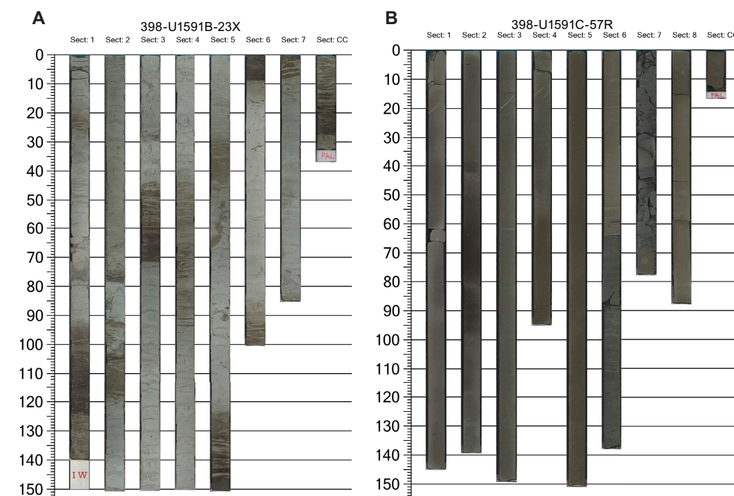
Figure F10. Core composites, Holes U1591B and U1591C. A. Cyclic intervals of ooze and organic-rich ooze (sapropelic ooze). B. Small proportion of organic-rich lithologies.
