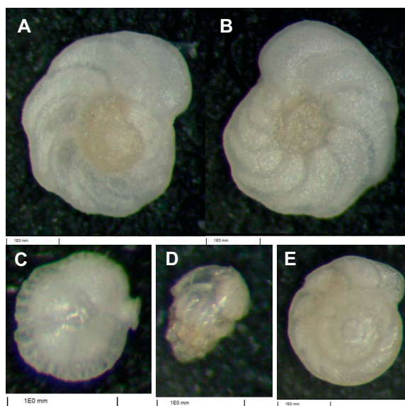
Figure F33. Benthic foraminifera, Hole U1591C. A, B. Cibicidoides wuellerstorfi (8R-CC, 14–16 cm); (A) umbilical view; (B) spiral view. C. Siphonina reticulata (13R-CC, 14–16 cm). D. Bulimina costata (39R-CC, 0–2 cm). E. Cibicidoides mundulus (9R-CC, 9–12 cm).
