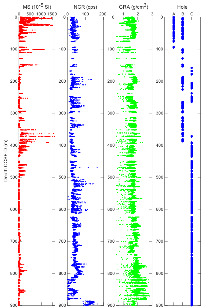
Figure F20. Splice for Site U1591 showing MS, NGR, and GRA density, as well as the respective spliced core interval from Holes U1591A–U1591C. cps = counts per second.
