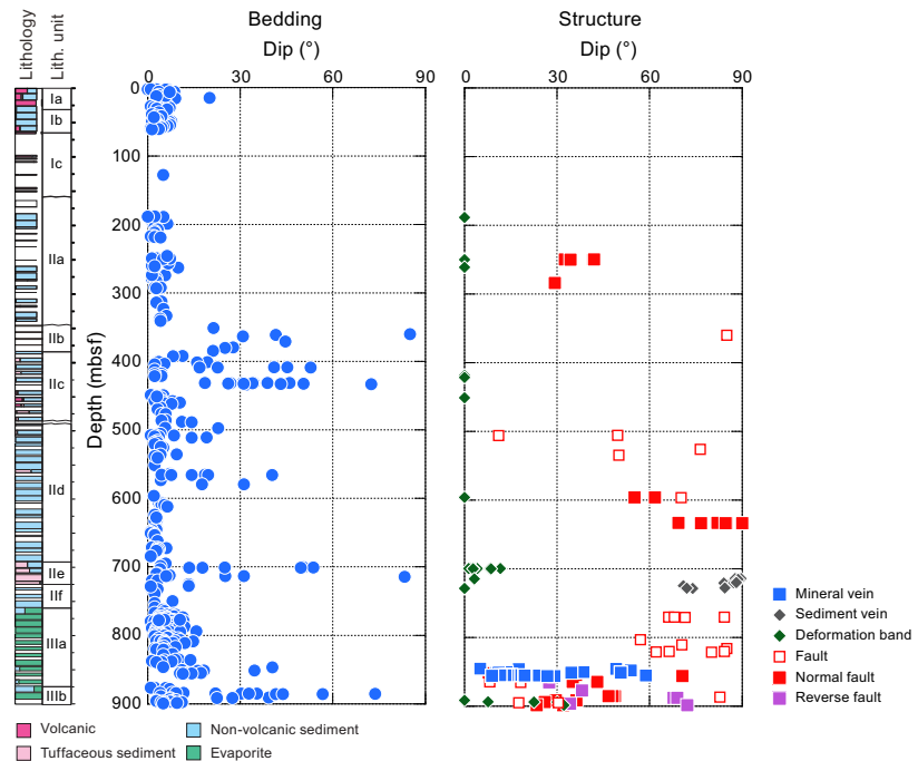
Figure F22. Dip data, Site U1591.
