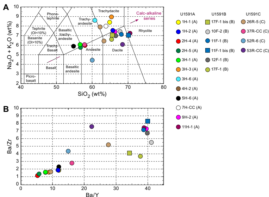
Figure F47. ICP-AES analyses of selected volcanoclastic units used to discriminate between potential volcanic sources, Site U1591. A. Total alkali vs. \text{SiO}_2 plot with the rock nomenclature of Le Maitre et al. (2002) overlain used for sample naming. Ol = olivine. B. Ba/Y vs. Ba/Zr plot used to correlate samples following Kutterolf et al. (2021).
