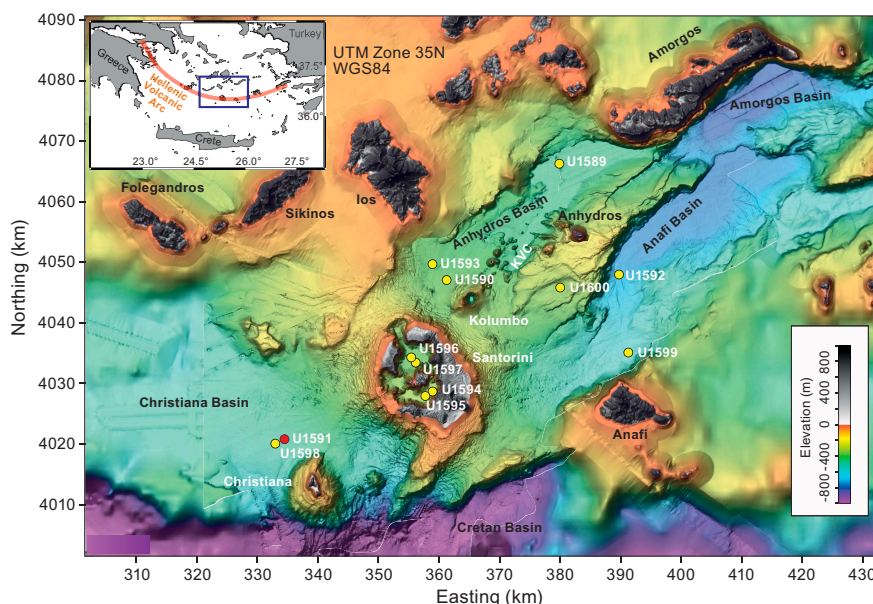
Figure F1. Site map. Red = Site U1591, yellow = other sites. Inset: location map. See Figure F1 in the Site U1589 chapter (Druitt et al., 2024) for citations for the swath data on which this map is based. KVC = Kolumbo volcanic chain.
