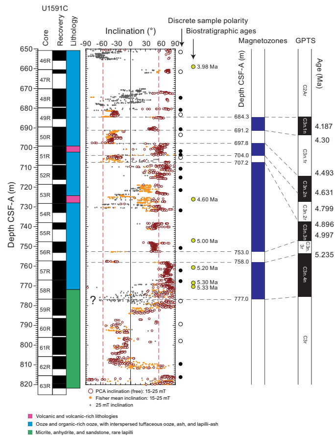
Figure F40. Archive-half section magnetic inclinations for interval 650–820 mbsf, Hole U1591C. Data are used to define magnetozones that are correlated to the geomagnetic polarity timescale (GPTS) of Gradstein et al. (2020). Red dashed lines = geocentric axial dipole inclinations expected at this site. Solid/open circles = normal/reversed polarity of discrete samples.
