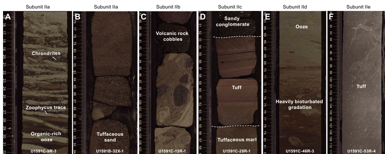
Figure F12. Representative lithologies from Unit II, Holes U1591B and U1591C. A, E. Cyclic repetitions of ooze/mud. B, D, F. Organic-rich (sapropelic) oozes/marl and muds/mudstone with minor ash and tuffaceous mud/sand. C. Sections in Subunit IIb contain volcanic rock cobbles.
