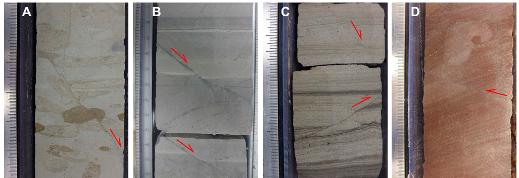
Figure F25. Small faults identified on split core surfaces, Hole U1591C. Arrows indicate the position of the faults and sense of shear direction. A, B. Normal faults identified just below slump layers (A: 40R-3, 33–45 cm; B: 12R-4, 77–88 cm). C, D. Reverse faults (C: 69R-3, 86–98 cm; D: 66R-6, 62–75 cm). Note in C a normal fault also developed.
