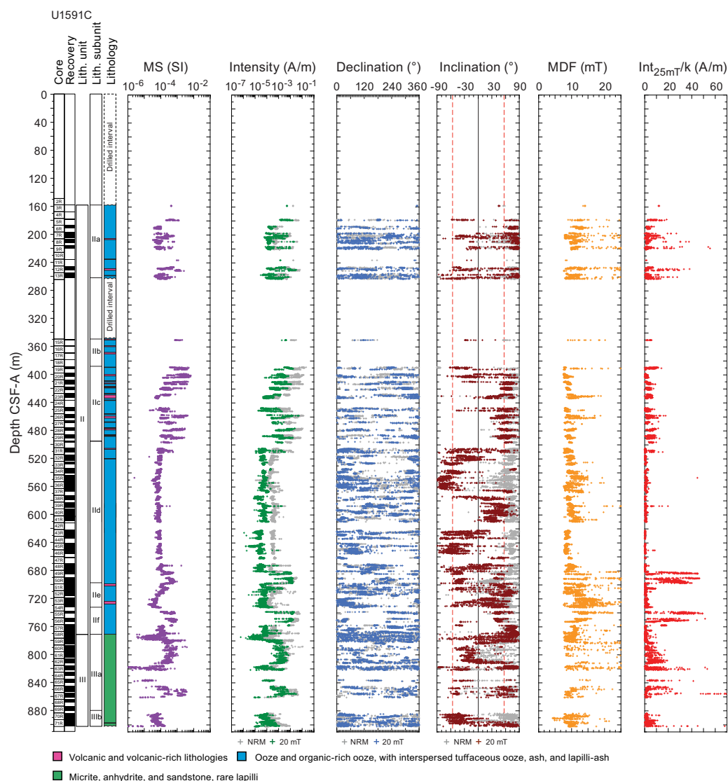
Figure F37. Archive-half section magnetic data, Hole U1591C. Red dashed lines = geocentric axial dipole inclinations expected at this site.
