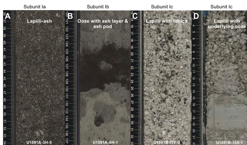
Figure F7. Representative volcanic lithologies from Unit I, Holes U1591A and U1591B. A. Ash layers. B. Ooze with ash. C, D. Lapilli layers. The ooze in D separates two large lapilli packages as shown in Hole U1591B in Figure F3.
