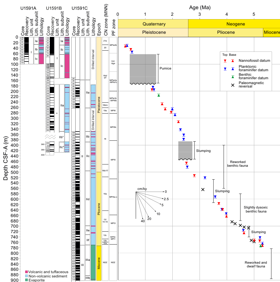
Figure F27. Age–depth plot, Holes U1591A–U1591C. Integrated biochronology and magnetostratigraphy are shown. CN = calcareous nannofossil, MNN = Mediterranean Neogene Nannoplankton, PF = planktonic foraminifer. Hiatuses correspond to periods of significant sediment remobilization. Biohorizons are listed in Tables T6 and T9. * = depth and recovery affected by slumped material.
