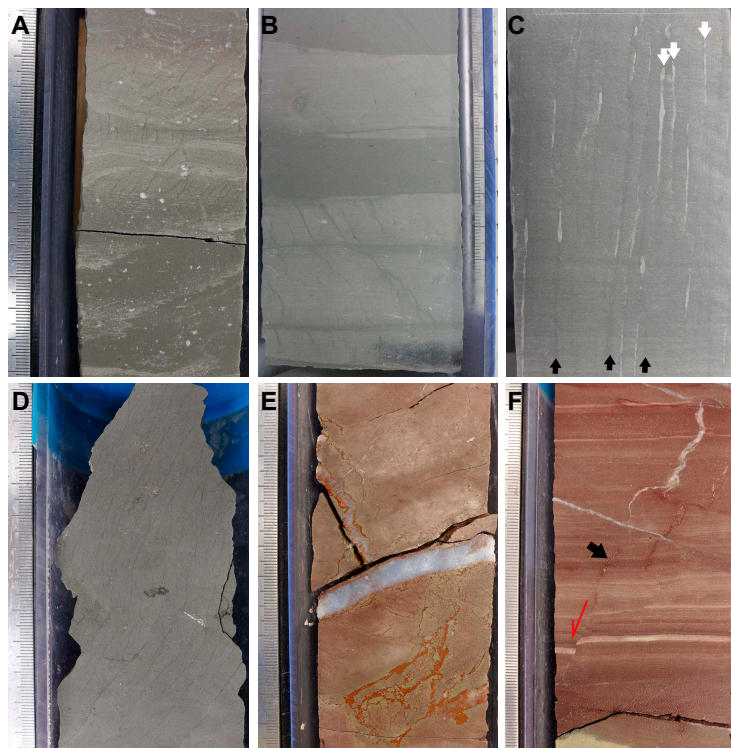
Figure F26. Sediment-filled veins in Units II and III, Hole U1591C. A–D. Typical occurrences of mud-filled vein structure in Unit II (A: 12R-1, 37–49 cm; B: 26R-4, 104–116 cm; C: 53R-2, 64–74 cm; D: 51R-CC, 0–13 cm). Note in C sand-filled veins (white arrows) apparently developed parallel to the mud-filled veins (black arrows) in the split-core section. E, F. Anhydrite veins developed in Unit III (E: 66R-1, 119–131 cm; F: 67R-2, 2–15 cm). Note small crystal growths (black arrow) along the normal fault (split arrow).
