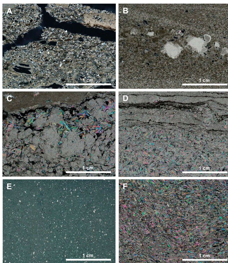
Figure F15. Evaporite lithologies from Unit III (XPL), Hole U1591C. A. Sandstone (58R-2, 6–9 cm). B. Sandstone with anhydrite nodules (58R-5, 63–66 cm). C. Laminated anhydrite alternating with micrite (58R-5, 115–118 cm). D. Laminated anhydrite alternating with algal mats and micrite (69R-1, 15–18 cm). E. Fine-grained anhydritic mudstone with crystals including feldspar, quartz, and biotite (71R-1, 90–93 cm). F. Coarse-grained anhydrite characterized by elongated anhydrite and gypsum crystals with interstitial micrite (71R-CC, 20–22 cm).
