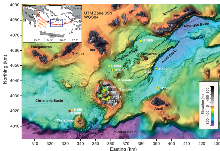
Figure F1. Site map. Red = Site U1598, yellow = other sites. Inset = location map. See Figure F1 in the Site U1598 chapter (Druitt et al., 2024a) for the swath data on which this map is based. KVC = Kolumbo volcanic chain.
