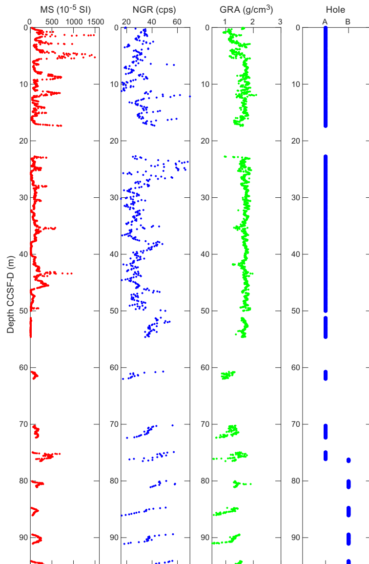
Figure F10. MS, NGR, and GRA density, Site U1598. For WRMSL data, see Physical properties .
