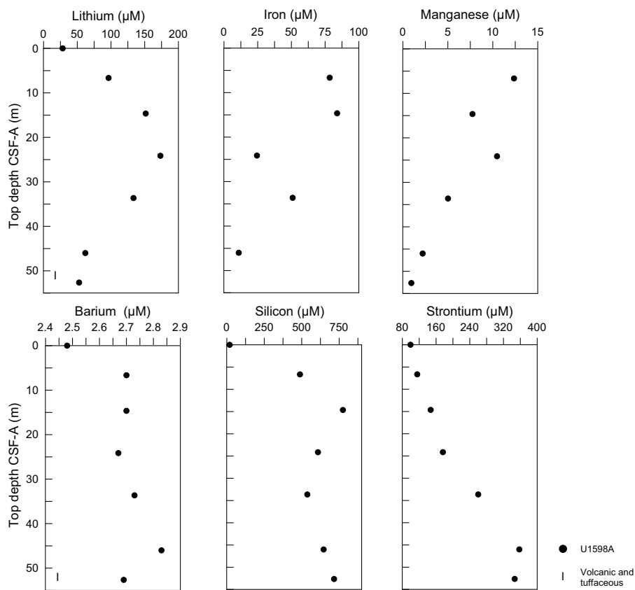
Figure F23. ICP-AES concentrations of Li, Fe, Mn, Ba, Si, and Sr in IW samples, Site U1598. Lithostratigraphic Unit I is described in Lithostratigraphy.
