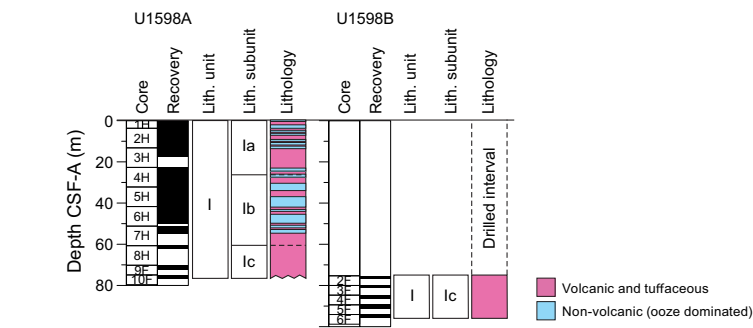
Figure F3. Lithostratigraphic summary, Site U1598. Unit color = dominant lithology.
