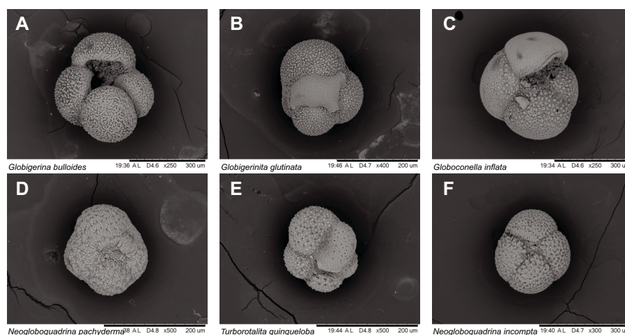
Figure F16. Planktonic foraminifera, Sample 398-U1598A-2H-CC, 0–3 cm. A. Globigerina bulloides . B. Globigerinita glutinata . C. Globoconella inflata . D. Neogloboquadrina pachyderma . E. Turborotalita quinqueloba . F. Neogloboquadrina incompta .
