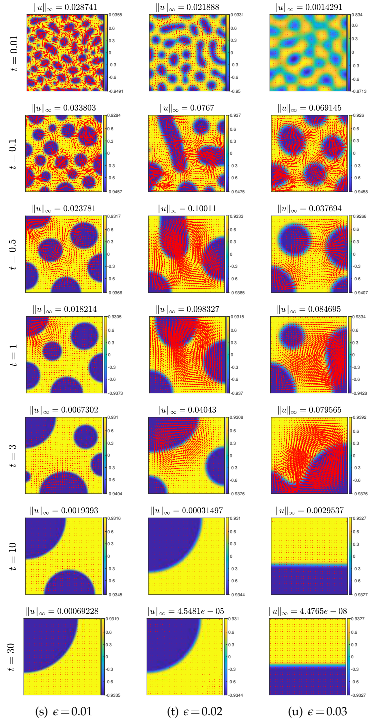
Figure 3: Numerical simulation of the coarsening process.
