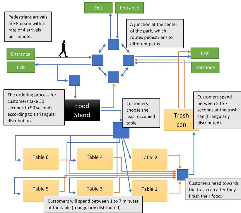
Figure 2: The logic of the hotdog stand simulation model (reprinted with permission from [20])
