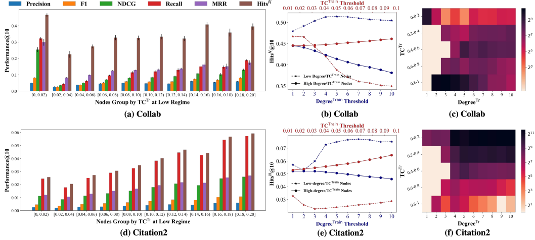
Figure 4: (a)/(d): The average LP performance of nodes with extremely low TC^{Train} on Collab/Citation2 almost monotonically increases as TC^{Train} increases. (b)/(e): Nodes with lower Degree Train surprisingly perform better than their higher degree counterparts (Blue curves). In contrast, non-concentrated nodes identified by owning lower TC^{Train} in most cases perform worse than their concentrated counterparts (Red curves). (c)/(f): As node Degree Train increases, the ratio of nodes owning higher TC^{Train} increases first and then decreases, corresponding to the observed first-increasing-and-then-decreasing performance trend in Figure 1(c)/(d).
