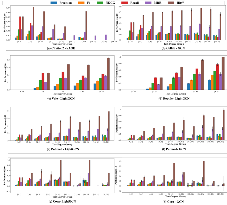
Figure 16: LP performance grouped by Degree Test for low Test-Degree nodes
