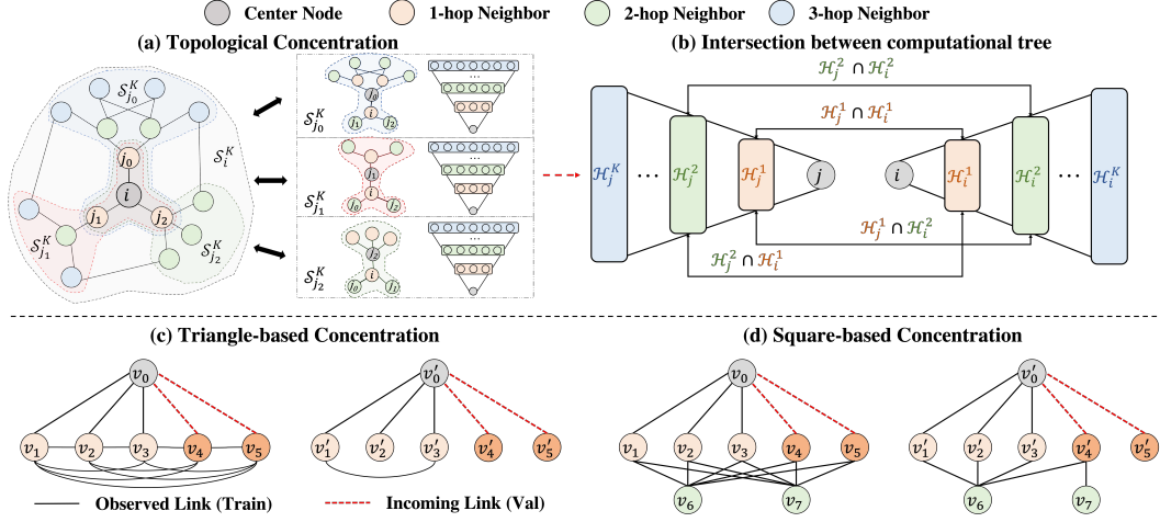
Figure 2: (a)-(b): v_i 's Topological Concentration: we calculate the average intersection between v_i 's computation tree and each of v_i 's neighbor's computation tree. The intersection between two computation trees is the ratio of the observed intersections to all possible intersections. (c)-(d): two specifications of TC, corresponding to social and e-commerce networks. A higher triangle/square-based concentration indicates more triangles/squares are formed among v_0 's local subgraph.
