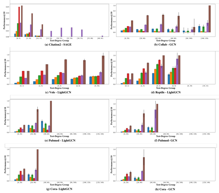
Figure 15: LP performance grouped by Degree Test for all nodes
