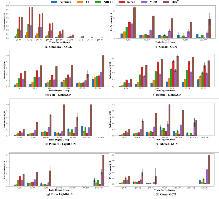
Figure 17: LP performance grouped by Degree Train for all nodes
