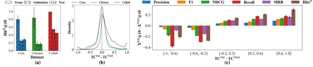
Figure 5: (a) Hits N @10 of predicting training/validation/testing edges on Cora/Citeseer/Collab. The gap between validation and testing performance is much bigger on Collab than on Cora/Citeseer. (b) Compared with Cora/Citeseer where edges are randomly split, the distribution of the difference between TC Val and TC Test shifts slightly right on Collab where edges are split according to time, indicating the interaction between training and testing neighbors become less than the one between training and validation neighbors. (c) As the gap between TC Val and TC Test increases for different nodes, their corresponding performance gap also increases, demonstrating TDS varies among different nodes even within the same graph.
