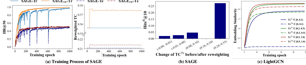
Figure 7: (a) Change of Hits@50 and Reweighted TC along the training process in SAGE. (b) Nodes with enhanced TC^{Train} exhibit higher performance. (c) Embedding similarity during LightGCN training increases faster and higher for nodes with higher TC^{Train} .
