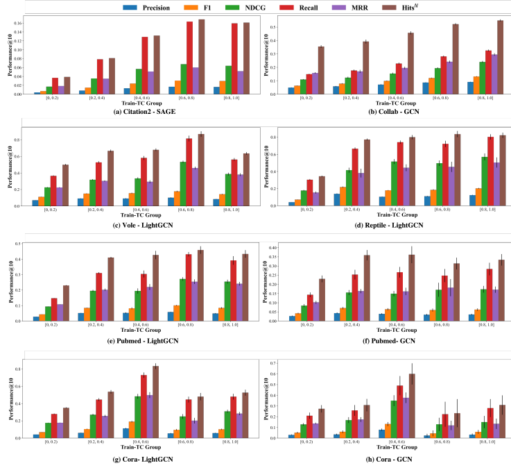
Figure 13: LP performance grouped by TC^{Train} for all nodes
