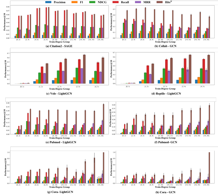
Figure 18: LP performance grouped by Degree Train for low Degree Train nodes
