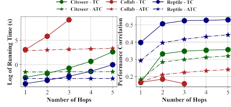
Figure 6: \text{ATC}^{\text{Train}} maintains a similar level of correlation to \text{TC}^{\text{Train}} while significantly reducing the computational time.
