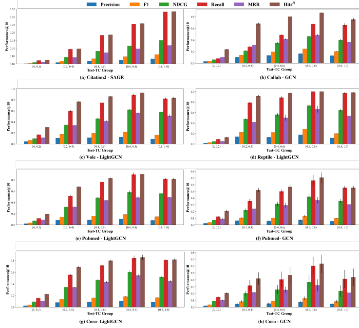
Figure 11: LP performance grouped by TC^{Test} for all nodes
