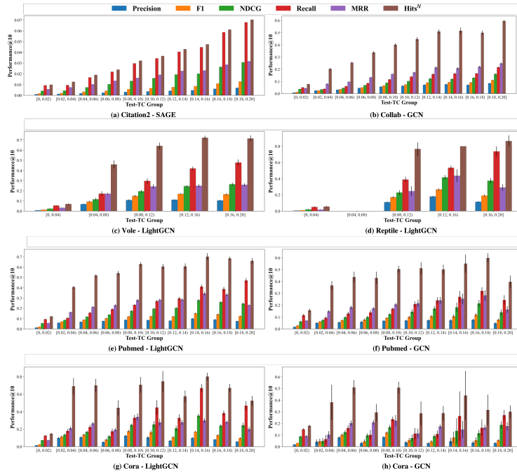
Figure 12: LP performance grouped by TC^{Test} for low TC^{Test} nodes
