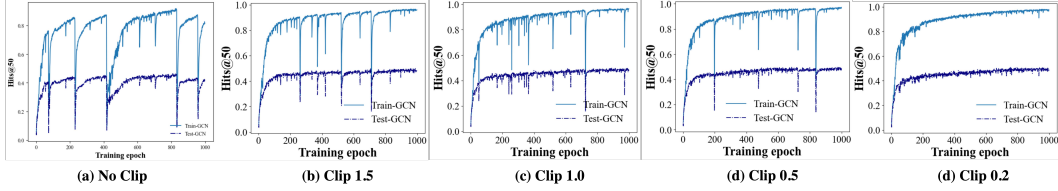
Figure 23: From left to right, we constrain GCN-based link predictor with fewer upper bounds by clipping using a lower threshold. We can see the number of performance fast downtrend decreases. We hypothesize that the loss landscape has several local minimums and hence by weight clipping with lower upper bounds, our learning step would be also smaller so that the model could not jump out of its origin local optimum and hence we end up with fewer fast downtrends.
