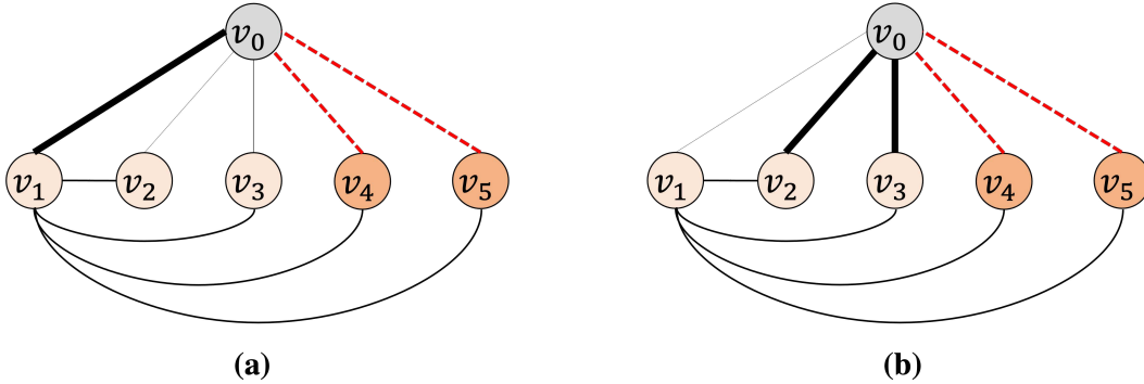
Figure 9: (a) Increasing the weight of neighbors that have more connections with the whole neighborhood while (b) increasing the weight of neighbors that have fewer connections with the whole neighborhood. (a) would increase the weighted TC while (b) would not
