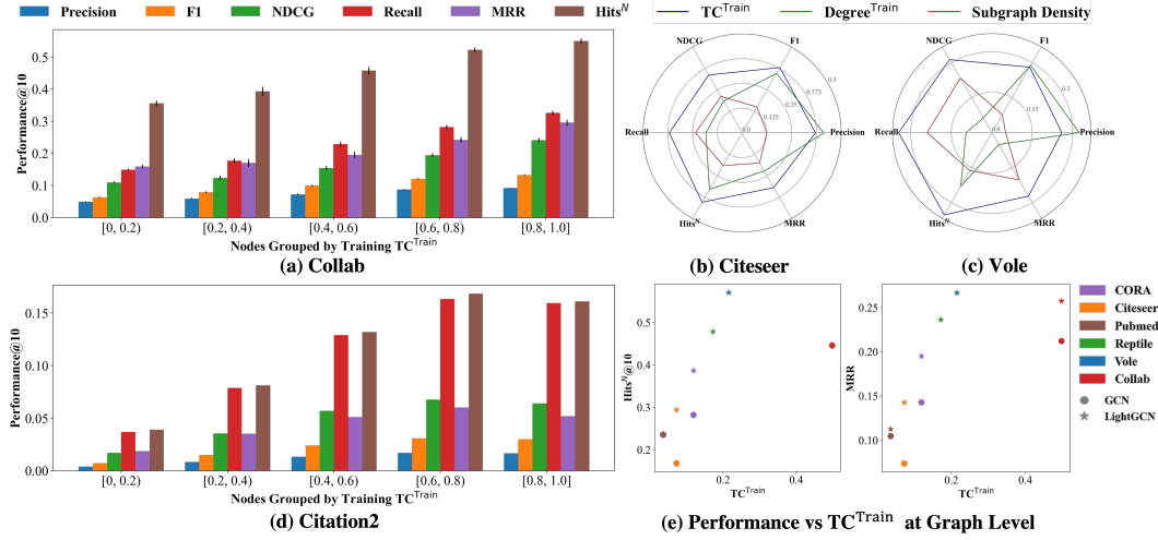
Figure 3: (a)/(d) : The average LP Performance of nodes on Collab/Citation2 monotonically increases as the TC^{Train} increases. (b)/(c) : TC^{Train} mostly achieves the highest Pearson Correlation with LP performance on Citeseer/Vole than Degree^{Train} and Subgraph Density metrics. (e) : LP performance is positively correlated to TC^{Train} across different network datasets. The deviation of Collab under both GCN and LightGCN baselines from the primary linear trend might be attributed to the duplicated edges in the network that create the illusion of a higher TC^{Train} .
