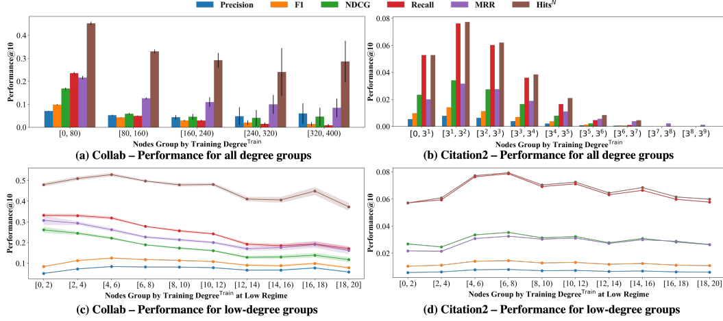
Figure 1: Average LP performance of nodes across different degree groups based on \text{Degree}^{\text{Train}} (i.e., node degree by training edges) on Collab/Citation2. In (a)-(b), Performance@10 does not increase as the node degree increases. In (c)-(d), few/lower-degree nodes do not perform worse than their higher-degree counterparts. Detailed experimental setting is included in Appendix F
