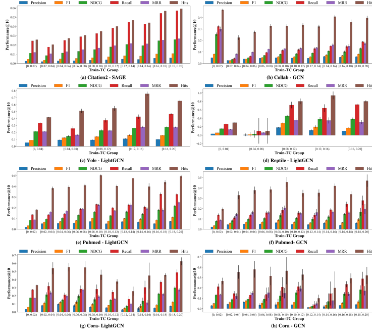
Figure 14: LP performance grouped by TC^{Train} for low TC^{Train} nodes
