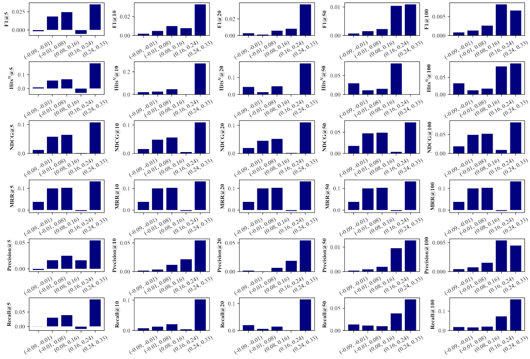
Figure 22: Relation between TC^{Train} and TC^{Test} on Collab by running SAGE
