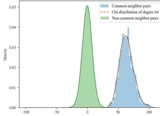
Figure 8: The distribution of the inner product between common neighbor pairs is statistically higher than that between non-common neighbor pairs.
