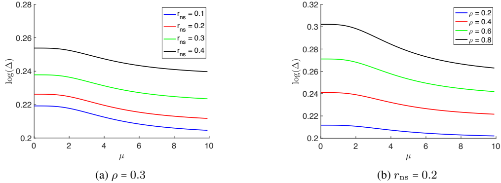
Figure 4: Behavior of gain \Delta in the generalization of the look-alike estimator \widehat{\theta}_L over min-norm estimator \widehat{\theta} as we vary \mu the energy of cluster centers.
