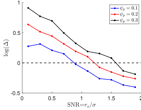
Figure 6: Behavior of gain \Delta versus SNR for the nonlinear model described in Section 6. At small SNR, we observe a positive gain (lower risk of look-alike estimator \hat{\theta}_L compared to \hat{\theta} ).
