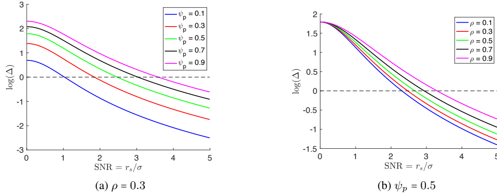
Figure 3: Behavior of gain \Delta in the generalization of the look-alike estimator \hat{\theta}_L over min-norm estimator \hat{\theta} as we vary \text{SNR} = r_s/\sigma . Here, \psi_d = 0.9 , \sigma = 1 , and we are in the underparametrized regime for both \hat{\theta}_L and \hat{\theta} .
