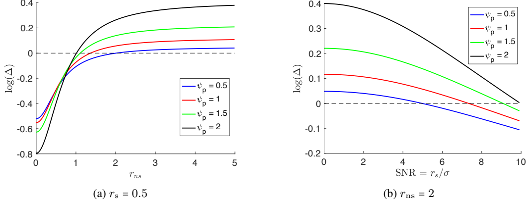
Figure 5: Behavior of gain \Delta versus r_{\text{ns}} and \text{SNR} = r_s/\sigma for several values of \psi_p . Here, \psi_d = 4 , \sigma = 0.1 , \rho = 0.3 , \mu = 5 , k = 5 . Here, we are in the overparametrized regime for both \hat{\theta}_L and \hat{\theta} .
