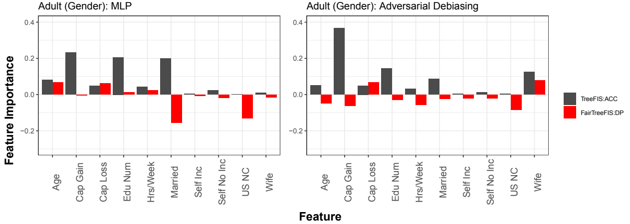
Figure 7: Interpretation of features for models with bias mitigation. The FairTreeFIS values show the difference in importance scores between a tree-based surrogate of a deep learning (two hidden layer MLP) model and a tree-based surrogate of a bias mitigation approach, deep learning adversarial debiasing method. Note that the “Married” feature has the most negative FairTreeFIS in the tree-based surrogate model, but is significantly less negative in the debiased model.
