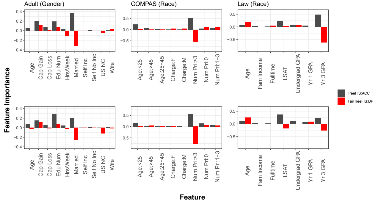
Figure 6: Global surrogate validation. The top row shows TreeFIS and FairTreeFIS results on a gradient boosting classifier for the Adult, COMPAS and Law datasets. The bottom row shows TreeFIS and FairTreeFIS results for a tree-based surrogate of a boosting classifier. The scores between the top and bottom rows are similar in magnitude and direction, indicating that our scores are effective when used to interpret tree-based global surrogates.
