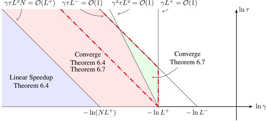
Figure 2: Different convergence conditions for local SGD.
