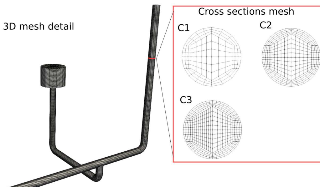
Figure 2: 3D mesh details showing the cross section resolutions for the cases C1, C2 and C3.
