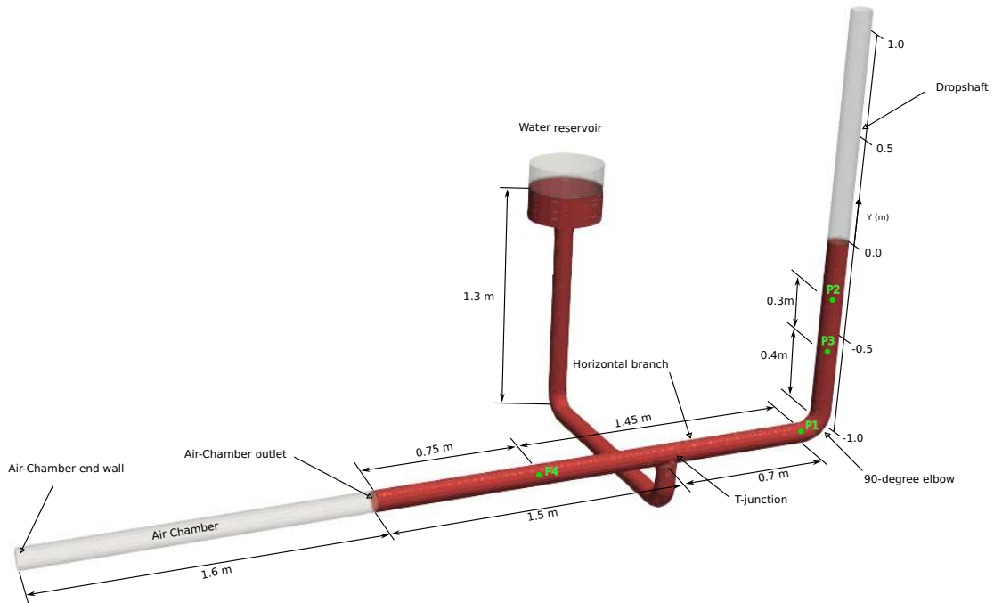
Figure 1: Computational domain for the flow problem simulated.
