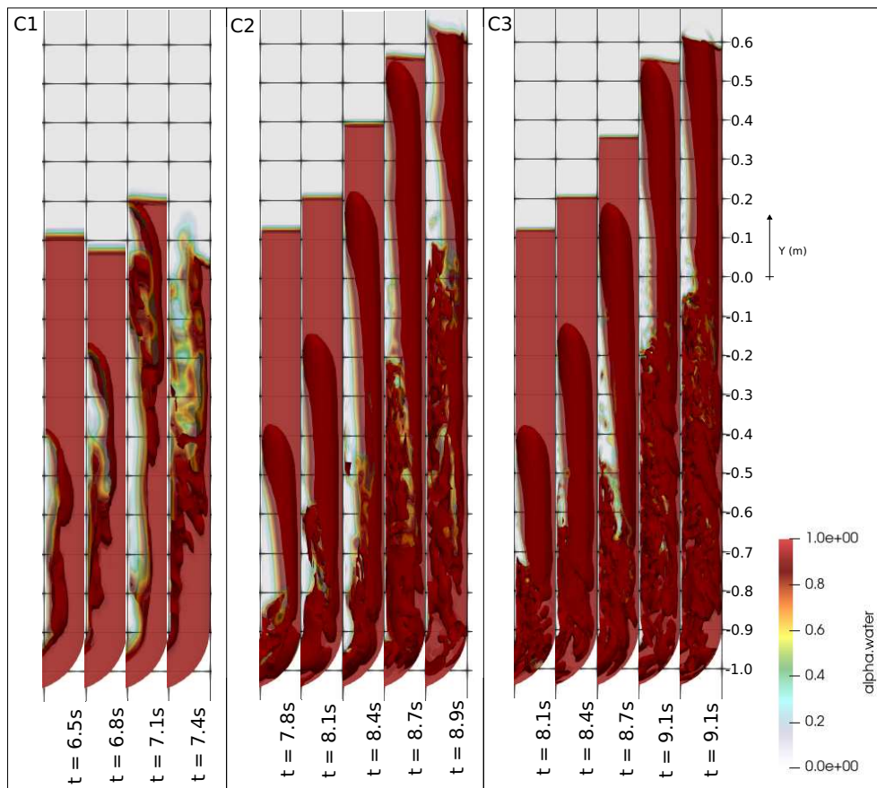
Figure 4: Air-pocket displacement visualization in the dropshaft for the cases C1, C2 and C3. The color scale pallet represents the water volume fraction \alpha .
